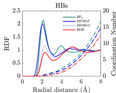
Fig. 8 RDFs of the HBs in the three DEEs.
