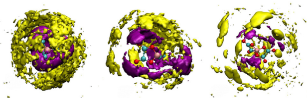
Fig. 7 SDFs for the: (a) LiBF 4 , (b) LiDFOB, and (c) LiBOB based DEEs showing lithium in purple and NMA in yellow around the anions.
