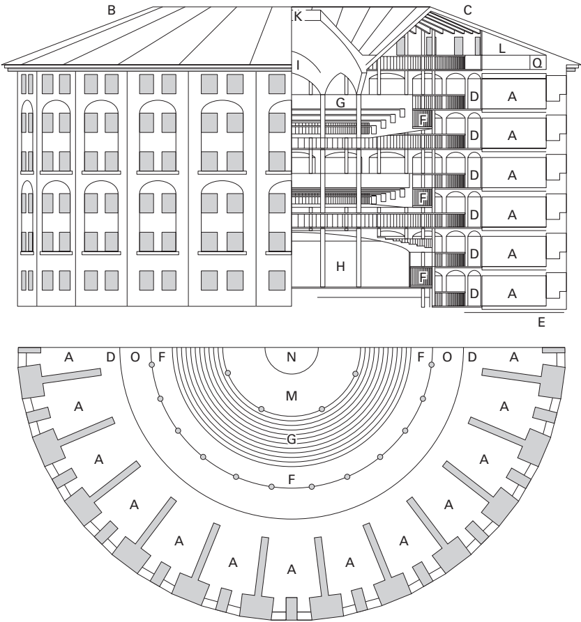
FIGURE A.1 Jeremy Bentham's panopticon; the influential solution for a prison where one guard could surveil a multitude of prisoners through an architectural innovation that creates particular properties of visibility.
