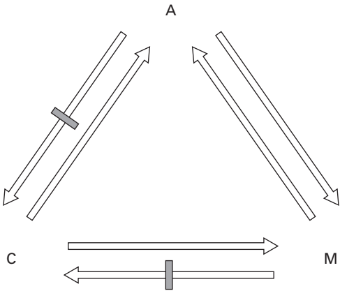
FIGURE 5.6 The theory of natural movement: attractor (A) and movement (M) may influence each other, but neither can influence configuration (C), at least not in the short run.
