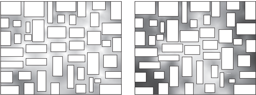
FIGURE 5.3 Metric and visual distance measured as universal distance, part III: analysis of universal visual distance in a gridlike bounded space, where small movements of the blocks cause large increases in universal visual distance but only marginal increases in universal metric distance (lighter shading indicates less visual universal distance).
