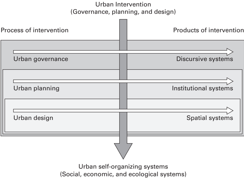
FIGURE 2.2 A model for the field of knowledge and practice in urban development. What is emphasized is that there are different professional practices that intervene in the self-organizing processes typical of cities, which do not so much demand knowledge about such processes in themselves as knowledge on the means to intervene in such processes typical for each profession, such as discourse , institutions , and spatial form , and more specifically how these means engage with and influence such processes.
