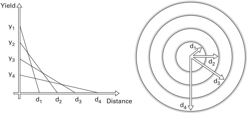
FIGURE 4.1 Johann Heinrich von Thünen’s 1826 model of land-use distribution around an agricultural market town depending on land rent and transportation costs (also used in modern bid-rent theory). Von Thünen set a high standard in capturing complex relations in simple geometry.
