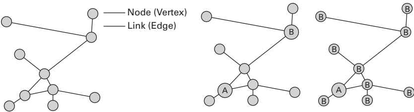
FIGURE 4.5 A network graph (left): representations of relations between entities as nodes (vertices) and links (edges). Regular distance (middle) is measured from location A to location B, and centrality (right) is measured as the mean distance from location A to all the other locations.
