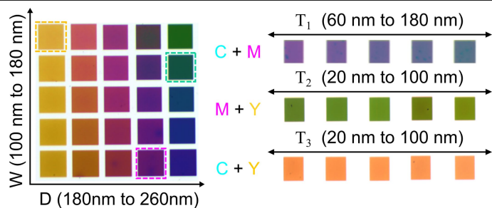
Extended Data Fig. 6 | CMY pixels in the air. The intermediate regions of CMY pixels contain all RGB pixels. By optimizing subpixel spacing ( T ), a blue pixel emerges when the CM subpixel distance is 100 nm, green at an MY subpixel distance of 60 nm, and red at a CY subpixel distance of 60 nm.
