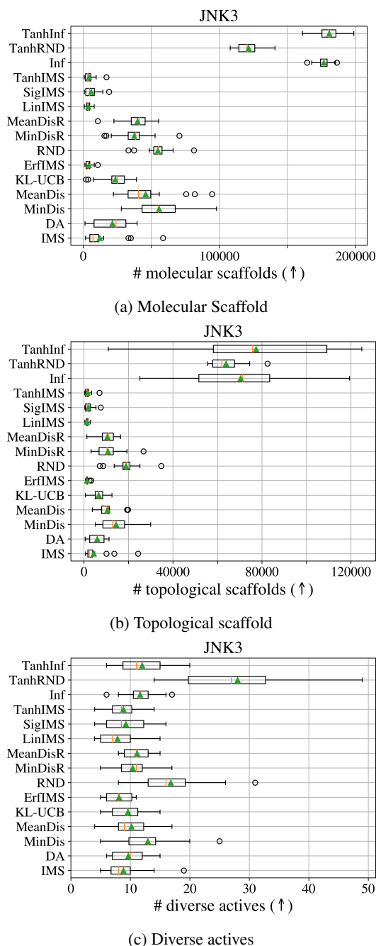
Figure 4: Evaluation of diversity on the JNK3 oracle. The boxplots compare the total number of molecular scaffolds, topological scaffolds and diverse actives after 2000 generative steps. Each boxplot displays the evaluation across 20 independent runs of each method, where the orange line and green triangle display the median and mean, respectively. Only active molecules are considered when computing the diversity metrics.
