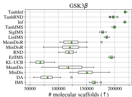
(a) Molecular scaffold
