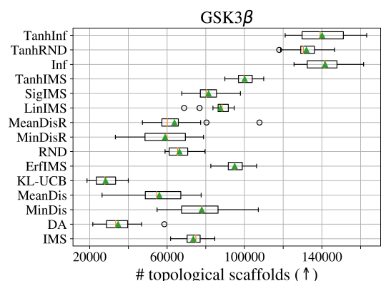
(b) Topological scaffold
