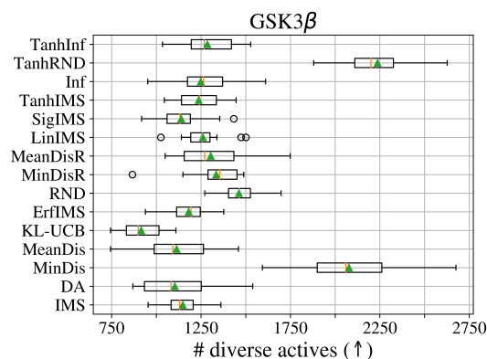
(c) Diverse actives
