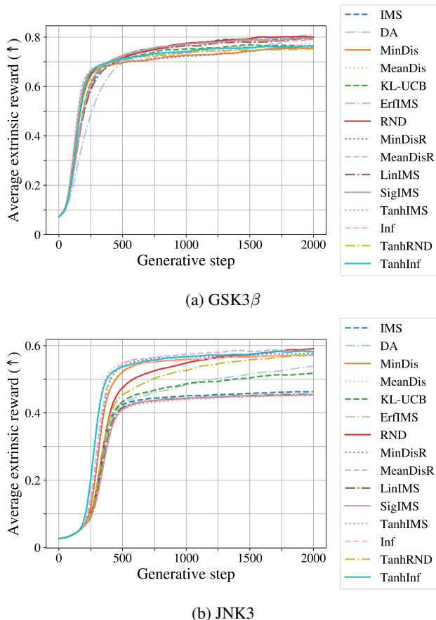
Figure 2: Average extrinsic reward (moving average using a window size of 101), over 20 independent runs, per generative step for both the GSK3 \beta and the JNK3 oracle.
