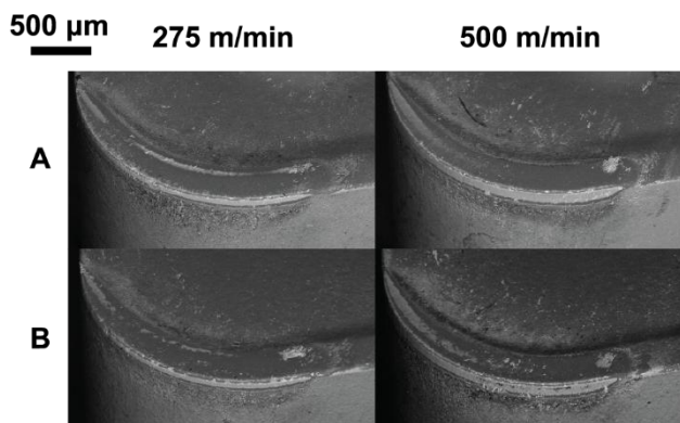
Fig. 6: Overview SEM images of worn inserts for both tool grades at cutting speeds 275 m/min and 500 m/min.
