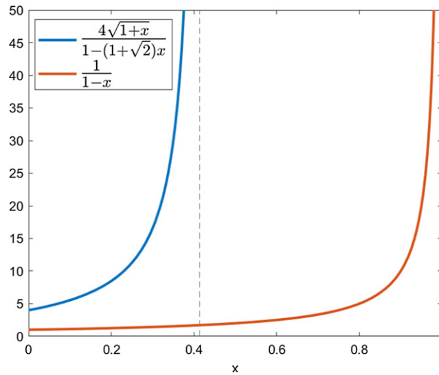
Figure 4. f_{\text{CGO}} in red and f_{\text{C}} in blue.
