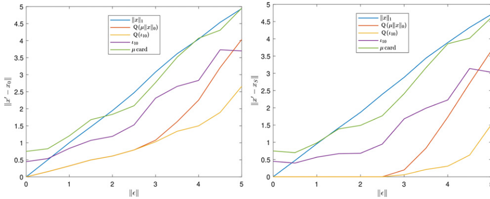
Figure 5. \|x' - x_0\|_2 (left) and \|x' - x_S\|_2 (right) versus \|\epsilon\|_2 for the 5 methods (3), (10), (11) and (15), (16) minimized using with FBS. The methods based on Q_2(\text{card}) and Q_2(\ell_{P_k}) work perfectly down to \text{SNR} \approx 4 .
