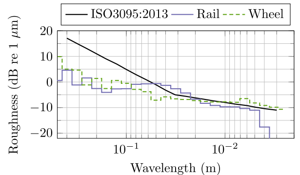
Figure 4. Average wheel and rail roughness spectra, in one-third octave bands.
