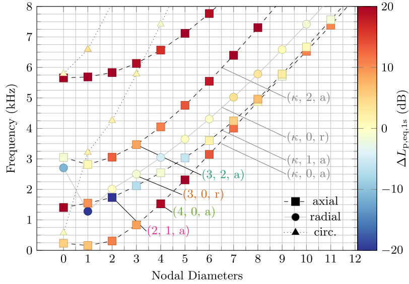
Figure 8. Dispersion diagram where each marker represents a mode of the wheel. The color indicates the difference in L_{p,eq,1s} between excitation at Node 1 and Node 2, where positive differences correspond to larger radiation for an excitation at Node 2.
