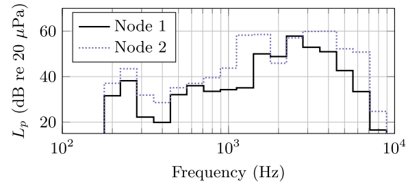
Figure 7. Total SPL for the two excitation positions.
