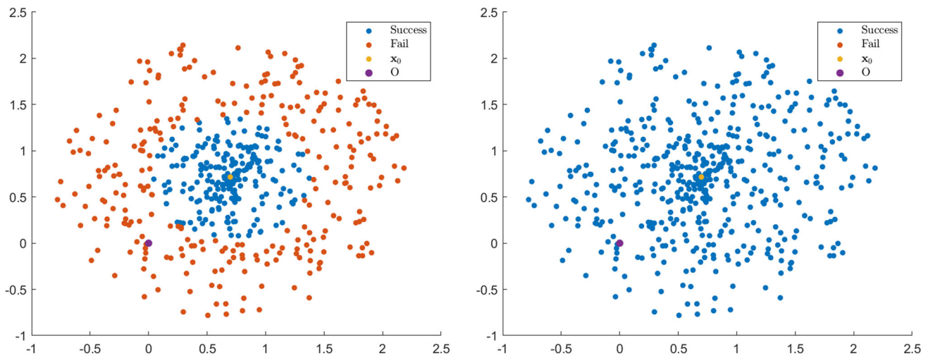
Fig. 6 Starting points clouds. The image on the left shows the outcome for the functional Q_2(\mu \|\cdot\|_0)(\mathbf{x}) + \|\mathbf{A}\mathbf{x} - \mathbf{b}\|^2 while the image on the right shows the outcome for (13)
