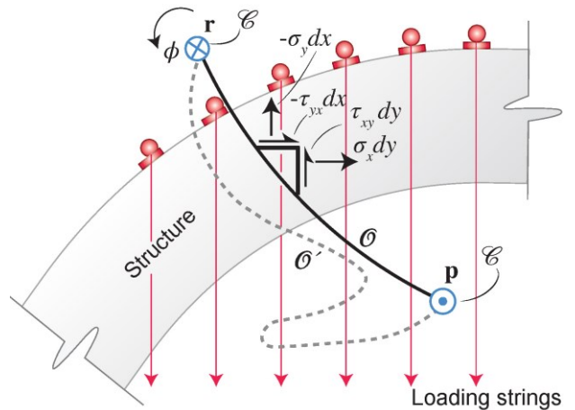
Figure 3: The Airy stress function \phi is the moment about \mathbf{r}
