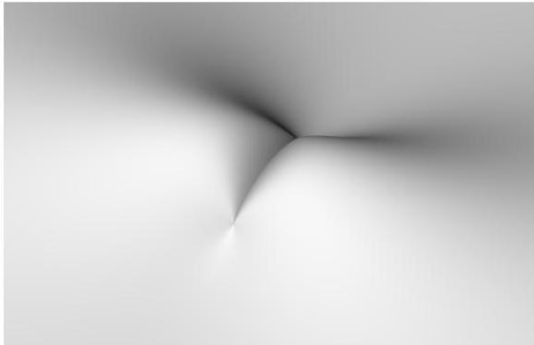
Figure 5: Airy stress function for two equal and opposite point loads in an elastic plate under plane stress. The fold in the surface corresponds to the concentrated force in the loading contraption producing the two loads. The curvature of the surface is the same on both sides of the fold, so the stress in the plate is continuous
