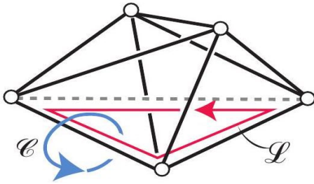
Figure 9: Triangular bipyramid. The loop \mathcal{L} in red is added for the dotted grey the loading jack
