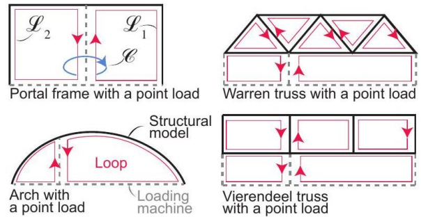
Figure 8: Structures formed of loops, with the loading contraptions shown dotted
