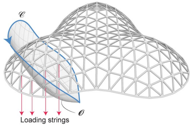
Figure 2: Shell cut by surface \mathcal{O} bounded by closed curve \mathcal{C}
