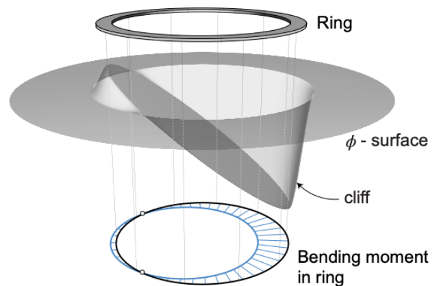
Figure 4: Airy stress function for ring carrying internal bending moments. The height of the 'cliff' gives the value of moment and the narrower the ring the steeper the cliff
