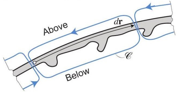
Figure 10: Section through a shell structure
