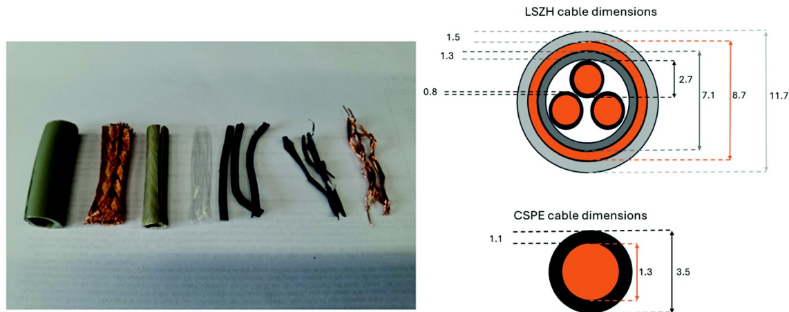
Figure 4. Dimensions of the cable layers for the LSZH and CSPE cables (all numbers in millimeter). To the left a photo of the LSZH cable layers. Note that layers four and six (counted from the right) on the photo are omitted from the figure (they are too thin to measure reliably and have no practical bearing on the dimensions).
