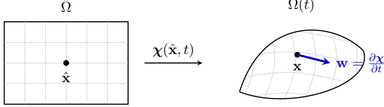
Figure 2: The ALE mapping \chi transports the computational mesh from the structured reference domain \hat{\Omega} to the physical domain \Omega(t) , inducing a mesh velocity \mathbf{w} at the spatial coordinates.
