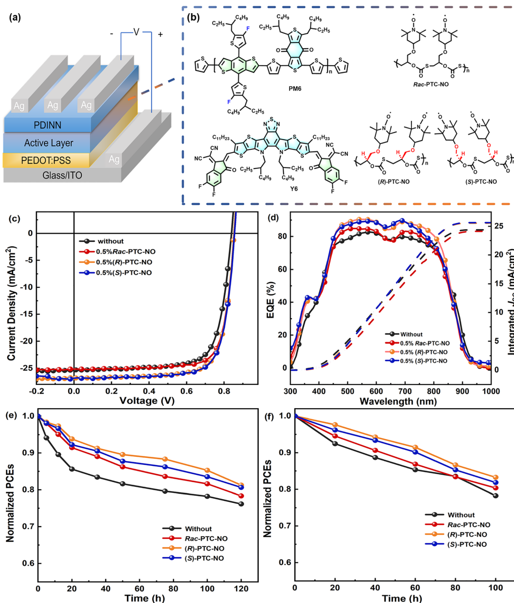
Fig. 2 (a) Device structure. (b) Chemical structures of PM6, Y6, Rac -PTC-NO, ( R )-PTC-NO, and ( S )-PTC-NO. (c) J/V , (d) EQEs, (e) photo-stability and (f) thermal stability of the NFA-OSC devices from PM6:Y6 films with and without 0.5 wt% of Rac -PTC-NO, ( R )-PTC-NO and ( S )-PTC-NO additives.
