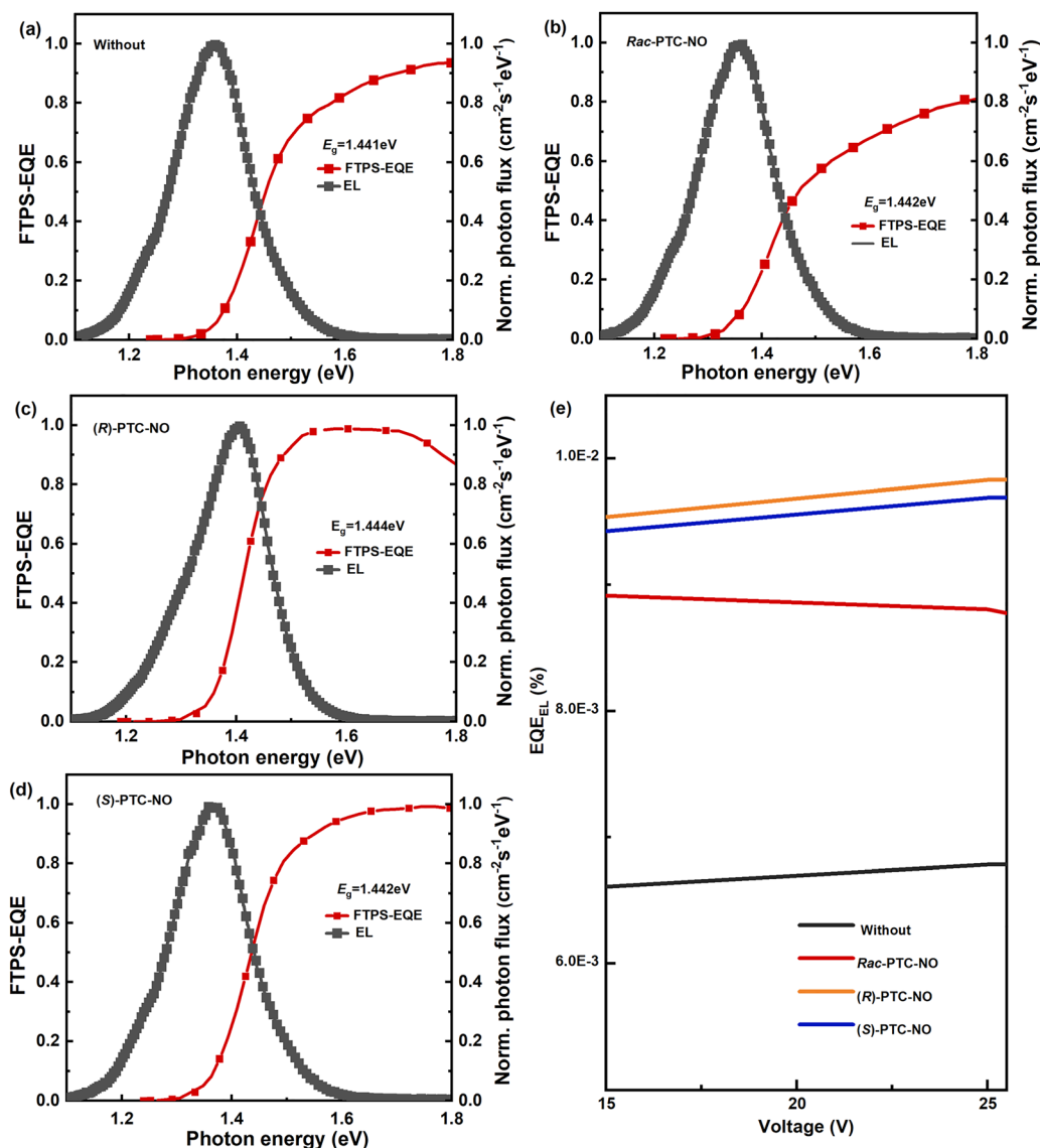
Fig. 5 EL, FTPS-EQE spectra (a)–(d) and \text{EQE}_{\text{EL}} (e) of NFAs-OSCs from the PM6:Y6 blends with and without 0.5 wt% of Rac -PTC-NO, ( R )-PTC-NO and ( S )-PTC-NO additives.
