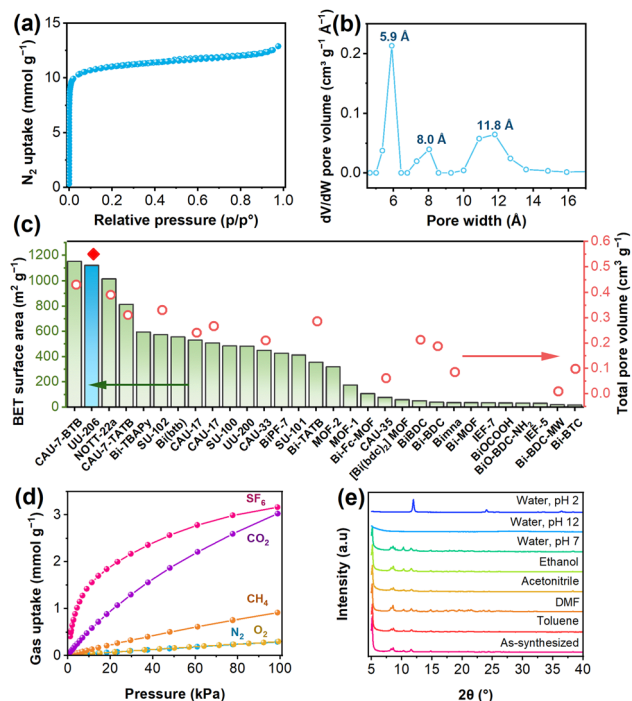
Fig. 2 (a) N_2 sorption isotherm recorded at -196^\circ\text{C} (or 77 K), (b) DFT pore size distribution, (c) comparison of the BET surface area and total pore volume of UU-206 and other Bi-based MOFs, (d) \text{CH}_4 , \text{CO}_2 , \text{N}_2 , \text{O}_2 , and \text{SF}_6 adsorption isotherms recorded at 20^\circ\text{C} , and (e) PXRD patterns of UU-206 after treatment in various solvents for 24 h.
