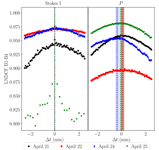
Fig. 9. LND CF between ALMA SPWs B1–B4 for all four days, showing total flux density (left) and polarized intensity (right). The dotted lines indicate the delays between SPWs B1–B4 retrieved from the LND CF.
