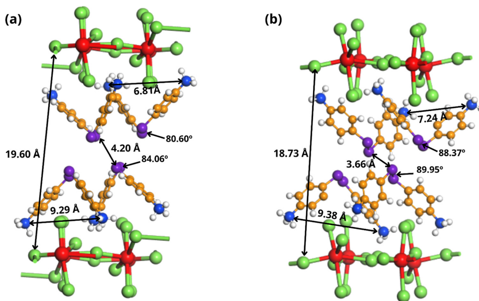
Fig. 4 Geometric optimization of the perovskite form proposed here, performed with the Biovia/Materials Studio 39 and Quantum Espresso 48,49 codes (panels (a) and (b), respectively). Colour code as in Fig. 1.
