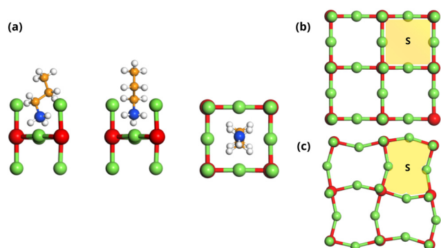
Fig. 2 Lateral and zenithal views of an Ruddlesden–Popper perovskite based on propylammonium, panel (a), with the available surface shown in panel (b). That area is the same even if the geometry is partially distorted, panel (c). Colour code as in Fig. 1.
