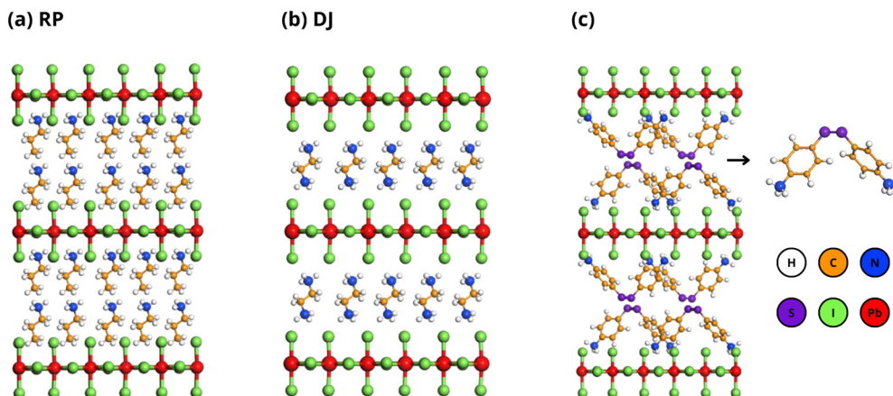
Fig. 1 Ruddlesden–Popper ( A'_{2n-1}B_nX_{3n+1} ) and Dion–Jacobson ( A''_{n-1}B_nX_{3n+1} ) perovskites, panels (a) and (b), respectively. A is an organic or inorganic cation, B is a divalent metal ( i.e. , Sn or Pb), X is a halogen anion ( i.e. , I or Br) and n is an integer ( n = 1, 2, 3, \dots ). In these plots A' is the propylammonium for the case of the RP perovskites, panel (a), while for the DJ phase A'' is the ethylenediammonium, panel (b). The perovskite form proposed here uses 4,4'-dithiodianiline molecules as spacers, panel (c). In all cases n = 1 .
