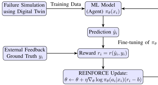
Fig. 1. RL based fine tuning of a pretrained agent \pi_\theta , originally trained using data generated by the DT. The policy network \pi_\theta(a_i|x_i) predicts optical amplifier failure conditions given input state of transmission parameters x_i , and receives reward r_i = r(\hat{y}_i, y_i) based on prediction accuracy with respect to ground truth y_i . The policy parameters \theta are updated using the REINFORCE rule with learning rate \eta : \theta \leftarrow \theta + \eta \nabla_\theta \log \pi_\theta(a_i|x_i)(r_i - b) , where b is a moving average baseline.
