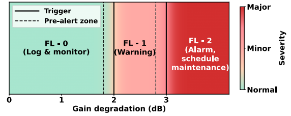
Fig. 3. Amplifier fault levels based on gain degradation.
