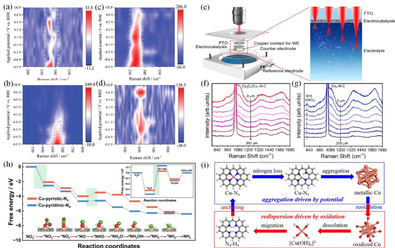
Fig. 9 (a and b) In situ Raman spectra of electrochemical nitrate reduction by p-CNCuLa and (c and d) p-CNCuLa-m, reproduced with permission. 109 Copyright 2025, Wiley-VCH. (e) Schematic diagram of the designed Raman cell. In situ Raman spectra of (f) Cu SACs/ \text{Co}_3\text{O}_4 and (g) Cu SACs, reproduced with permission. 110 Copyright 2024, Springer Nature. (h) Gibbs free energy diagram of electroreduction of nitrate and water dissociation by Cu-pyridinic-N 4 and Cu-pyrrolic-N 4 , reproduced with permission. 111 Copyright 2024, Elsevier. (i) Transformation between Cu-N 4 structures and Cu 0 nanoparticles, reproduced with permission. 113 Copyright 2022, American Chemical Society.
