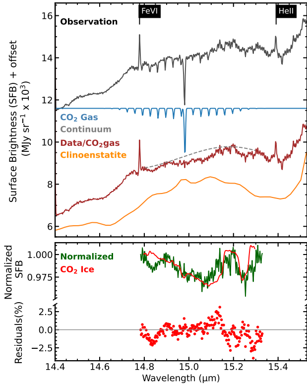
Fig. 1. Detection of CO 2 ice and gas. The overplotted black curve shows the JWST/MIRI spectrum at the position indicated by the dot in Fig. A.1. The uncertainties on the surface brightness are \sim \pm 40 MJy sr -1 . The best-fit gas-phase model ( T_{\text{gas}} = 30 K and \log N = 16.8 cm -2 ) is shown in blue. We divided out this model, resulting in the brown curve. The orange curve shows a single-temperature model for clinoenstatite emission. The dashed gray line shows the continuum we adopted to analyze the ice band. The green curve shows the normalized spectrum using that continuum. The red curve shows a laboratory spectrum for CO 2 ice (CO:CO 2 2:1 ice mixture at 80 K); and the bottom panel shows the residuals between the normalized spectrum (green) and the ice model (red).
