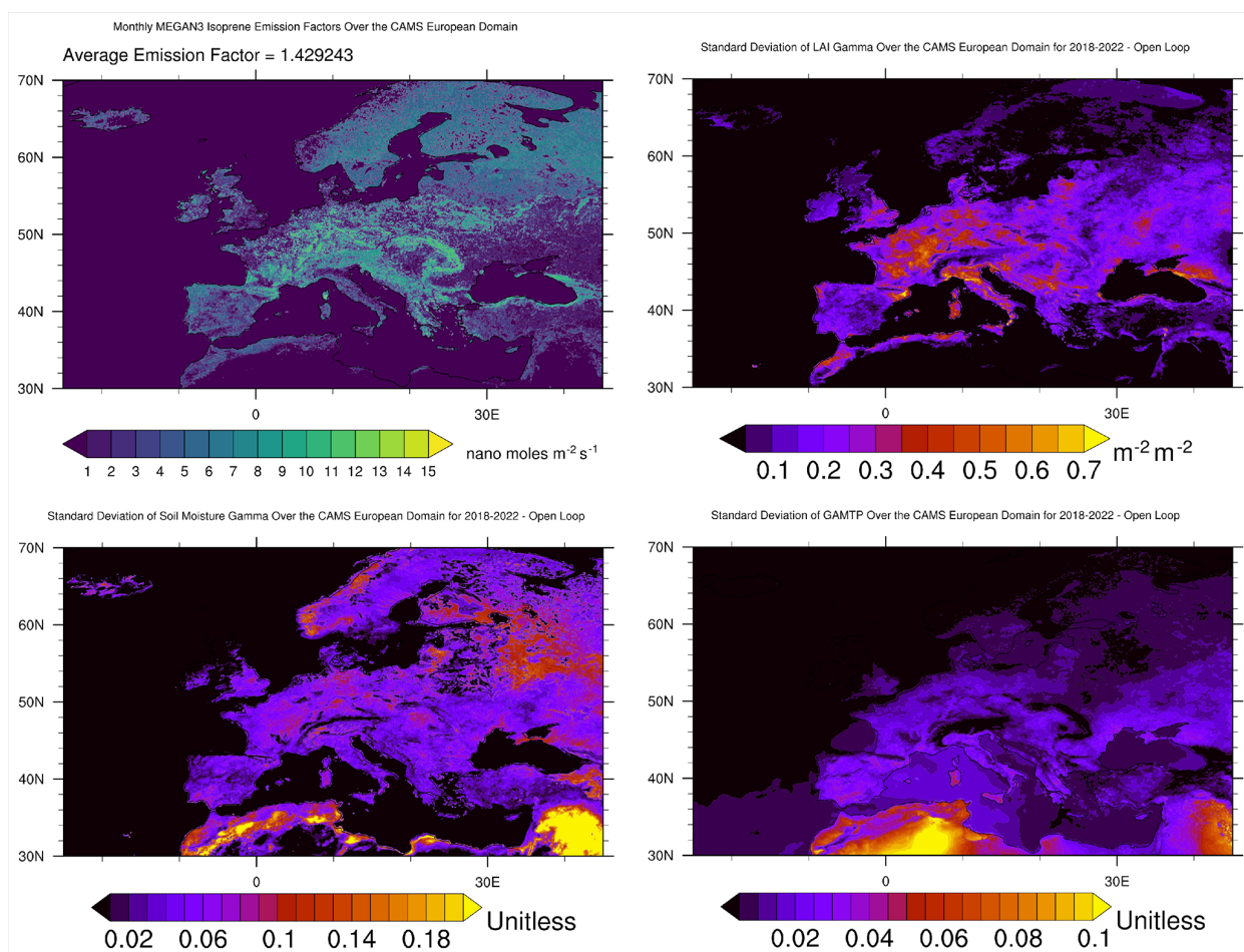
Figure 7. Maps of the MEGAN3.0 EFP isoprene emission factors in units of \text{nmol m}^{-2} \text{s}^{-1} (top left), the LAI gamma in units of \text{m}^{-2} \text{m}^{-2} (top right), the soil moisture gamma (unitless) (bottom left), and the temperature-radiation gamma in the bottom right.
