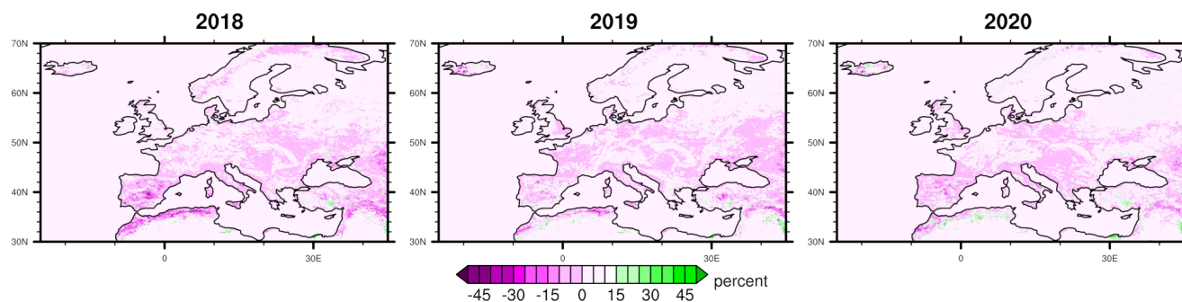
Figure 14. Maps of annual mean isoprene emissions (units of \text{kg m}^{-2} \text{s}^{-1} ) calculated using the SURFEX-MEGAN3.0 LAI analysis configuration of SURFEX (top-row), the difference between the LAI analysis minus the open-loop configurations (middle-row), and the percentage difference between the LAI analysis minus open-loop over the period 2018–2020. The panels show each year over this time period moving sequentially from 2018 to 2020 from left to right. The top-row colour bars indicate increasing mean isoprene emissions as the colours transition from pale yellow to dark green. The middle-row colour bars indicate the difference in annual mean isoprene emissions between the LAI-analysis and open-loop configurations with red colours indicating larger annual mean open-loop emissions and green indicating larger LAI-analysis based emissions. The bottom-row colour bar indicates the percentage difference in mean annual isoprene emissions between the LAI-analysis and open-loop with green indicating larger LAI-analysis based emissions and red indicating larger open-loop based emissions. The annual total mass of isoprene emissions (units of Tg) are shown above each plot in the top-row and the differences in annual total mass of isoprene emissions are shown above each plot in the middle-row.
