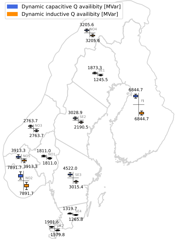
Fig. 2 Distributions of hourly available dynamic reactive power compensation in the Nordics from generators in the current system (2022). Availability is grouped by bidding zone and annual maximum availability is labelled.
