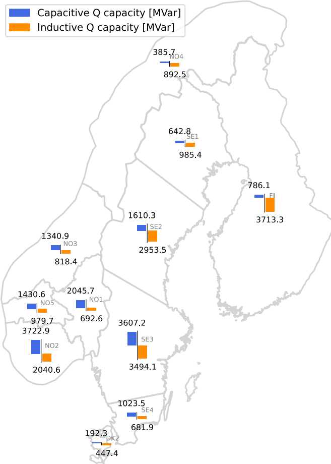
Fig. 1 Required steady-state reactive power capacities in the Nordics for the current system (2022). Capacities are grouped together by bidding zone.
