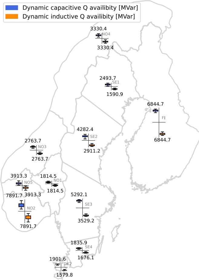
Fig. 3 Distributions of hourly available dynamic reactive power compensation in the Nordics from generation in the current system (2022) assuming changed grid codes requiring STATCOM operation (see Section 2.3.2). Availability is grouped by bidding zone and annual maximum availability is labelled.
