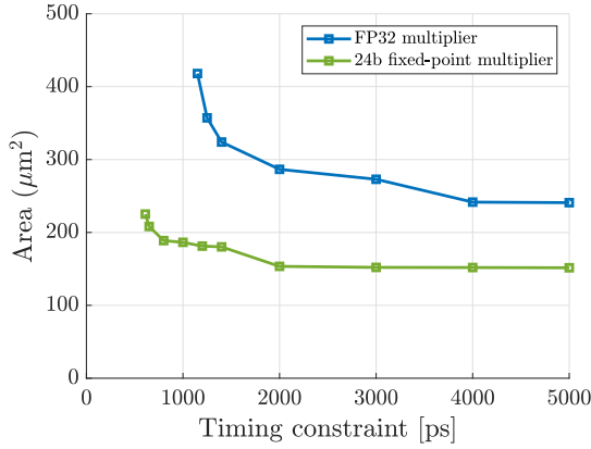
Fig. 2: Area of an FP32 multiplier vs a 24-bit fixed-point multiplier, as function of timing constraint.
