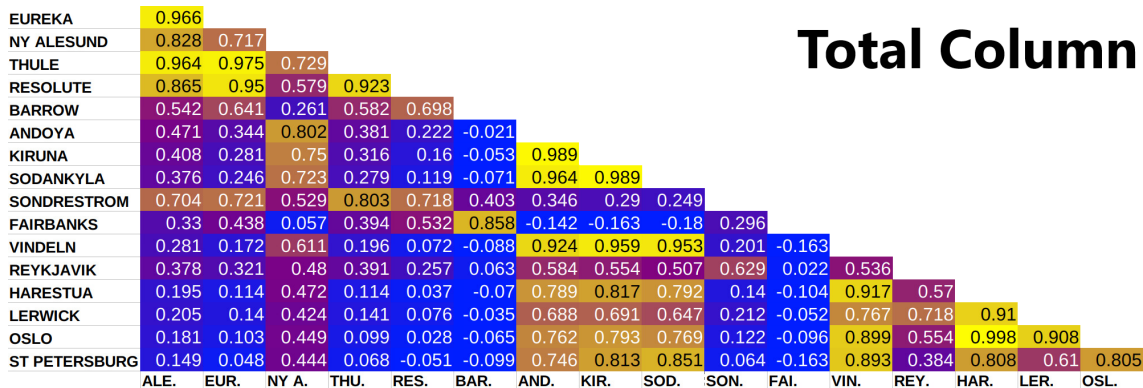
Figure A2. CAMS correlation table for the total column of ozone.
