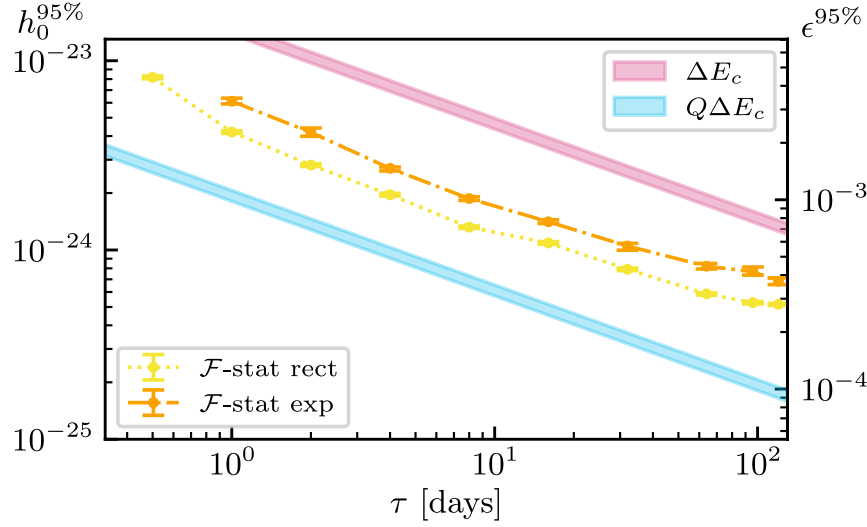
Figure 10. Upper limits from the transient \mathcal{F} -statistic search in terms of strain amplitude h_0^{95\%} (left-hand axis) and NS ellipticity \epsilon^{95\%} (right-hand axis) as functions of the signal duration parameter \tau . Results are included for both signals with constant amplitude (“rect”), as per Equation (8), and for exponentially decaying signals (“exp”), as per Equation (9). The same indirect energy limits are shown for comparison as in Figure 5, corresponding to Equation (17) with Q = 1 (magenta) and Q \approx 0.017 (sky blue).
