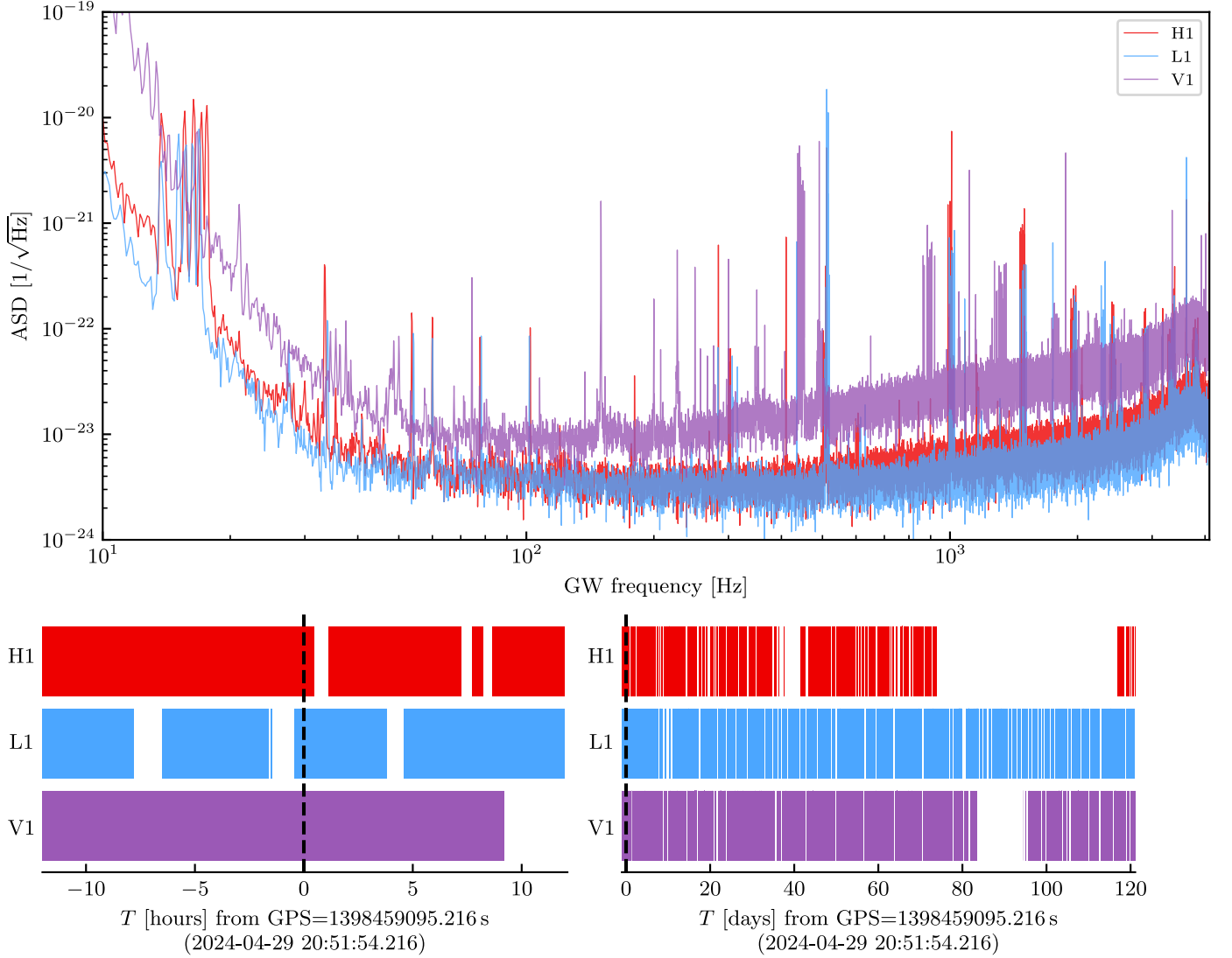
Figure 2. Top panel: GW detector sensitivities within T_{\text{gl}} \pm 20 s around the Vela glitch on 2024 April 29 in terms of their ASDs (computed with the Welch method in gwpy , D. M. Macleod et al. 2021). Bottom left panel: GW data availability over 24 hr around the glitch, as used for the burst searches in Section 4. Bottom right panel: LIGO data availability for the four following months, as used in the long-duration searches in Section 5. Virgo data is not used in either type of search. The glitch time is highlighted in the two bottom panels with a vertical dashed line.
