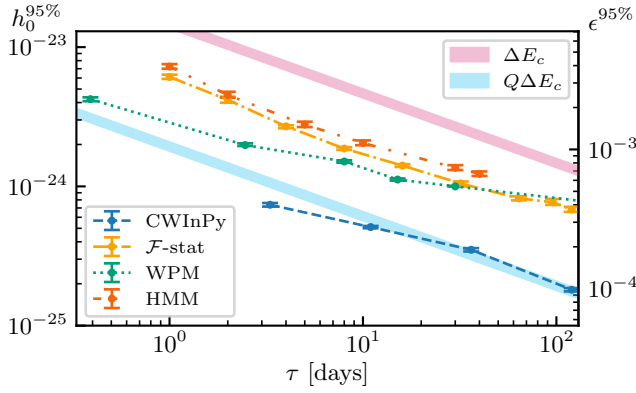
Figure 5. Selected upper limits at 95% confidence from the four CW-like postglitch searches, in terms of initial strain amplitude (left-hand axis) and NS ellipticity \epsilon (right-hand axis), both defined at the start of signals with exponentially decay parameters \tau . The results were chosen to illustrate how upper limits scale with the strictness of prior assumptions built into each search configuration. The CWInPy results have the strictest constraints (fixed frequency evolution and constrained orientation angles), while the three other results are for narrow-band searches, with \mathcal{F} -statistic results marginalized over all durations, WPM results for search configurations optimized at each \tau point, and HMM results for T_{\text{coh}} = 9 hr. For comparison, GW emission at the characteristic energy scale \Delta E_c from Equation (3) is shown as the magenta shaded band near the top, while the sky-blue shaded band further down shows the emission if the GW energy output is suppressed by a factor Q \approx 0.017 , as in G. Yim & D. I. Jones’s (2020) transient mountain model.
