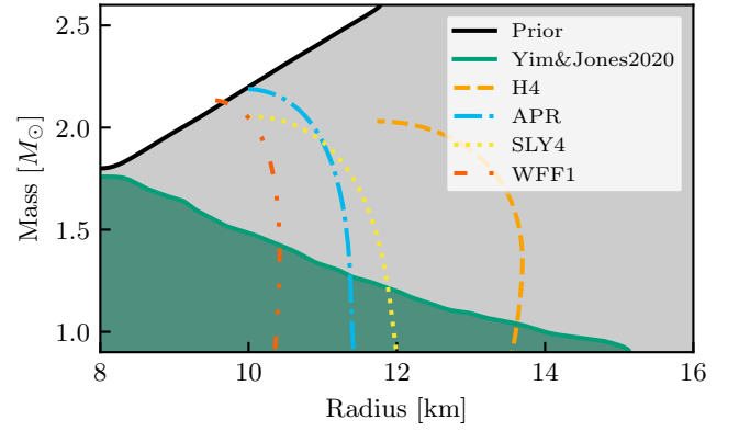
Figure 7. NS mass and radius regions for which the Vela pulsar could have emitted GWs according to G. Yim & D. I. Jones’s (2020) model after its 2024 glitch, but without our searches detecting them (within the green shaded region at the lower left, at 90% confidence). This is compared to the assumed prior ranges (larger black contour) and to mass–radius curves for some example equations of state (R. B. Wiringa et al. 1988; A. Akmal et al. 1998; F. Douchin & P. Haensel 2001; B. D. Lackey et al. 2006), for which allowed NS configurations would lie along each curve. Here, we fixed F_{\text{CW}} = 0.017 to match the healing parameter Q defined in Equation (7) and arbitrarily chose F_{\text{fmode}} = 0.8 (which has little effect). We see that the Yim & Jones model is only compatible with our nondetection for smaller mass and radius ranges.
