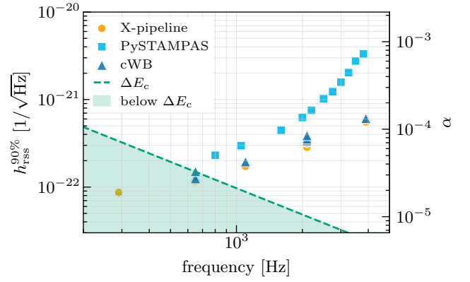
Figure 4. h_{\text{rss}}^{90\%} at a detection threshold of 3\sigma ( p -value 10^{-3} ) for the three GW burst searches (circle, square, and triangle markers), shown against the frequency of damped sinusoids signals. For cWB and X-pipeline, multiple markers at fixed frequencies denote different damping times (see Table 2), which do not affect the sensitivity drastically. Strains corresponding to the characteristic energy \Delta E_c of the glitch from Equation (3) are shown as the dashed green line and GW emission would be consistent with it in the shaded region below. The right-hand vertical axis shows the f -mode amplitude \alpha that would correspond to a given h_{\text{rss}} level. See Section 6.1 for interpretation of these results in terms of \Delta E_c and \alpha .
