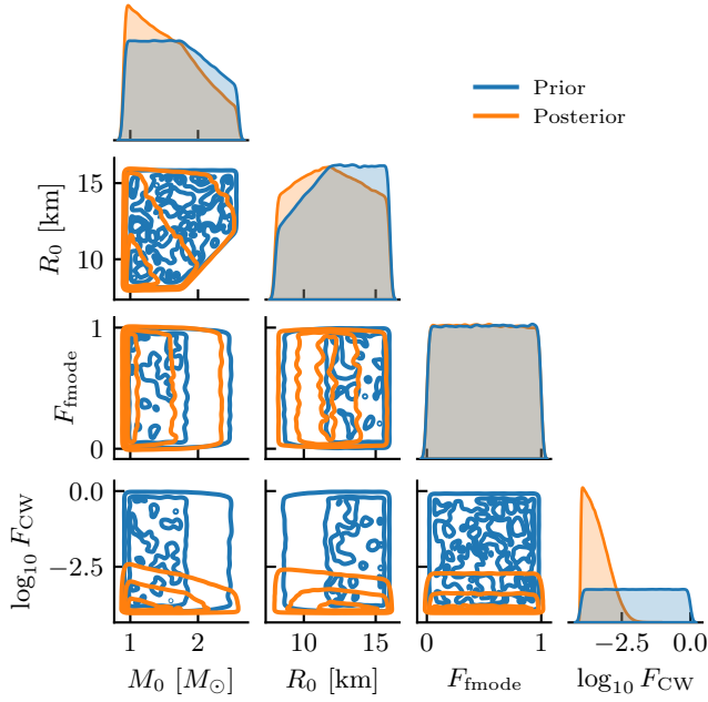
Figure 6. Prior and posterior distributions of NS mass, radius, and energy fractions F_{\text{fmode}} and \log_{10}(F_{\text{CW}}) under the assumption that GWs from both a short-duration f-mode and a long-duration transient mountain scenario were emitted but not detected. After including the search results, there is little effect on the allowed f-mode energy in the physically motivated region F_{\text{fmode}} < 1 but a measurable effect on the allowed CW energy ( F_{\text{CW}} ). Contours show 10%, 50%, and 90% credible intervals.
