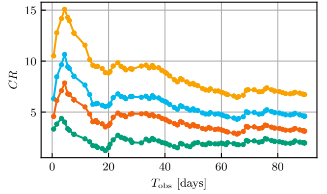
Figure 11. CR as a function of the observing window for the multi- \tau signal model and using the optimal segment duration T_{\text{seg}}^{\text{best}} = 96000 s. The plot has been obtained by injecting simulated signals into L1 data with four different signal amplitudes (going from the bottom to the top curve: [2.1, 4.2, 6.3, 8.4] \times 10^{-24} ). The “optimal” observing window corresponds to the maximum of the CR, which is nearly independent of the signal amplitude, taking place at T_{\text{obs}}^{\text{best}} \simeq 5.5 days.
