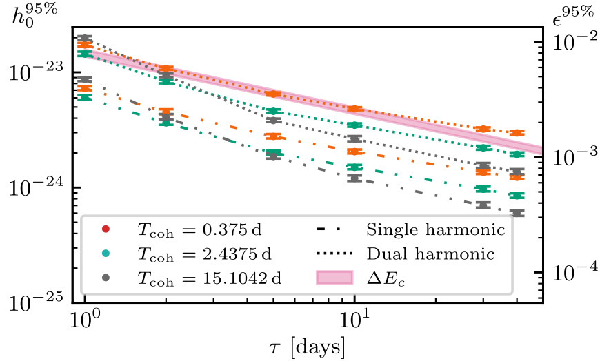
Figure 14. Upper limits on long-transient GWs from Vela inferred by the single (dashed–dotted lines) and dual-harmonic (dotted lines) HMM analyses as a function of the exponential signal decay time parameter \tau . Upper limits are expressed in terms of strain amplitude h_0^{95\%} (left axis) and NS ellipticity \epsilon^{95\%} (right axis). The magenta shaded comparison band labeled \Delta E_c corresponds to Equation (17) with Q = 1 .
