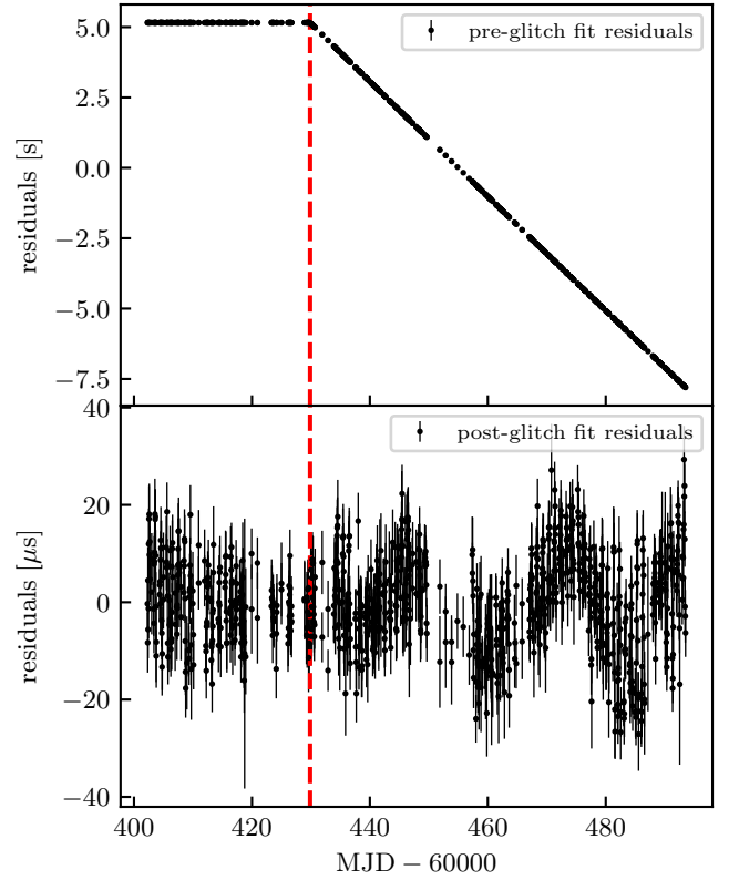
Figure 1. Top panel: Vela pulsar radio timing residuals before fitting for the 2024 April 29 glitch. Bottom panel: Timing residuals after fitting for the glitch with the parameters shown in Table 1.
