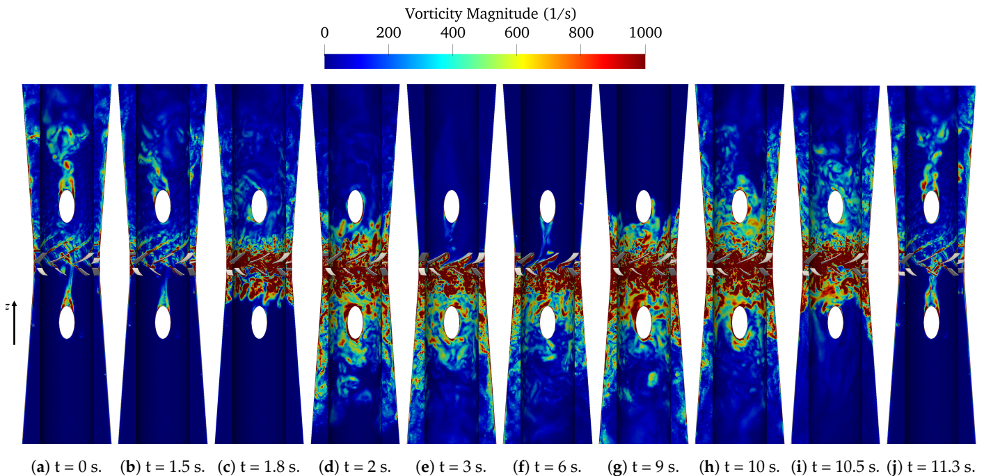
Figure 10. Zoomed-in view of the vorticity magnitude at various time steps during the transient sequences in pump mode. The results are displayed on a meridional plane and a cylinder (midpoint radius between hub and shroud) cutting the domain. The preferred flow direction is from bottom to top in pump mode.
