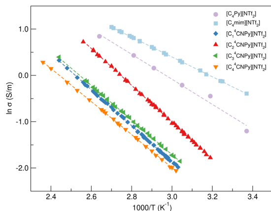
Fig. 4 Arrhenius plots of conductivity ( \ln \sigma vs. 1000/T , 313–420 K) for the neat ILs; [C_1^4\text{CNPy}][\text{NTf}_2] (blue), [C_2^4\text{CNPy}][\text{NTf}_2] (red), [C_3^4\text{CNPy}][\text{NTf}_2] (green), and [C_4^4\text{CNPy}][\text{NTf}_2] (orange), with dashed lines showing logarithmic fit of the data as a guide to the eye. Data for the reference ILs, [C_4\text{Py}][\text{NTf}_2] and [C_2\text{mim}][\text{NTf}_2] , are shown for comparison.
