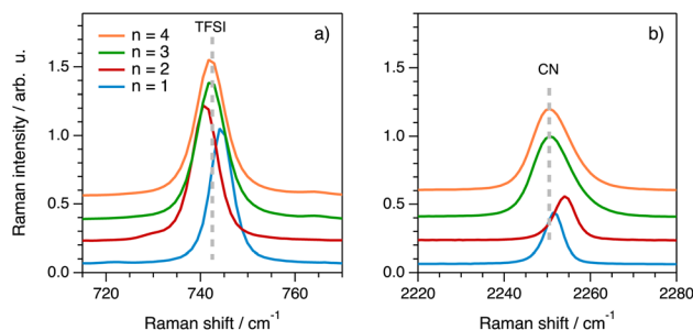
Fig. 10 Raman stretching signals from [\text{NTf}_2]^- anion asymmetric stretch at ca. 740 \text{cm}^{-1} (a, left) and the [C_n^4\text{CNPy}]^+ cation nitrile stretch at 2250 \text{cm}^{-1} (b, right).
