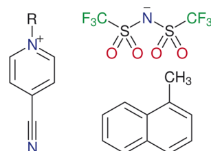
Fig. 1 Structures of the ionic liquid cation, [C_n^4\text{CNPy}]^+ ( n = 1-4 ), anion, [\text{NTf}_2]^- , and 1-methylnaphthalene (1-MN).
