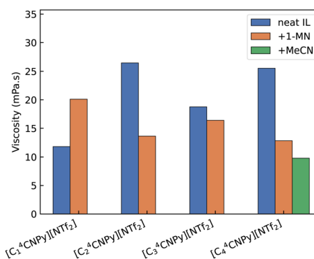
Fig. 6 Viscosities of neat ionic liquids (blue), IL : 1-MN mixtures (orange) and [C_4^4\text{CNPyl}][\text{NTf}_2] : MeCN (green) at 358 K (data extrapolated from the viscosity profiles in Fig. 5 for n = 1 and 2, and [C_4^4\text{CNPyl}][\text{NTf}_2] : MeCN) showing the relative changes, with the expected increase in viscosity with cation size (as n increases) and the competing impacts of CT-association leading to an increase in viscosity compared to the neat IL ( n = 1 ) through to a significant overall decrease in viscosity ( n = 4 ) albeit, reduced compared to the effects of the pure diluent, MeCN.
