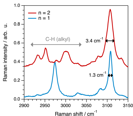
Fig. 12 Raman spectra in the region of alkyl and ring C–H stretching modes, for the samples [\text{C}_1^4\text{CNPpy}][\text{NTf}_2] (blue) and [\text{C}_2^4\text{CNPpy}][\text{NTf}_2] (red).
