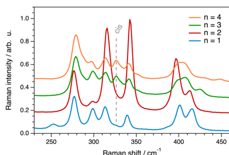
Fig. 9 The anion conformation region of the Raman spectra (250–450 \text{cm}^{-1} ) for neat [C_n^4\text{CNPy}][\text{NTf}_2] ILs under 785 nm laser excitation showing the characteristic signatures for trans [\text{NTf}_2]^- anions in solid [C_1^4\text{CNPy}][\text{NTf}_2] and [C_2^4\text{CNPy}][\text{NTf}_2] and a bands deriving from both cis and trans conformers in the liquids, [C_3^4\text{CNPy}][\text{NTf}_2] and [C_4^4\text{CNPy}][\text{NTf}_2] .
