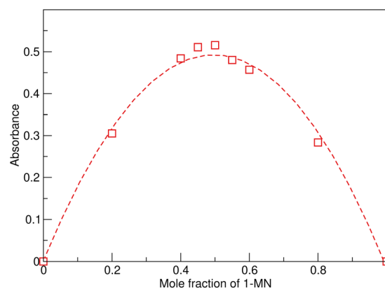
Fig. 2 Job's plot analysis showing maximum absorbance in the UV-vis spectrum at 375 nm from formation of the 1 : 1 CT complex between [C 1 4 CNPyl][NTf 2 ] and 1-MN in MeCN with total concentration of IL and 1-MN of 0.1 M.
