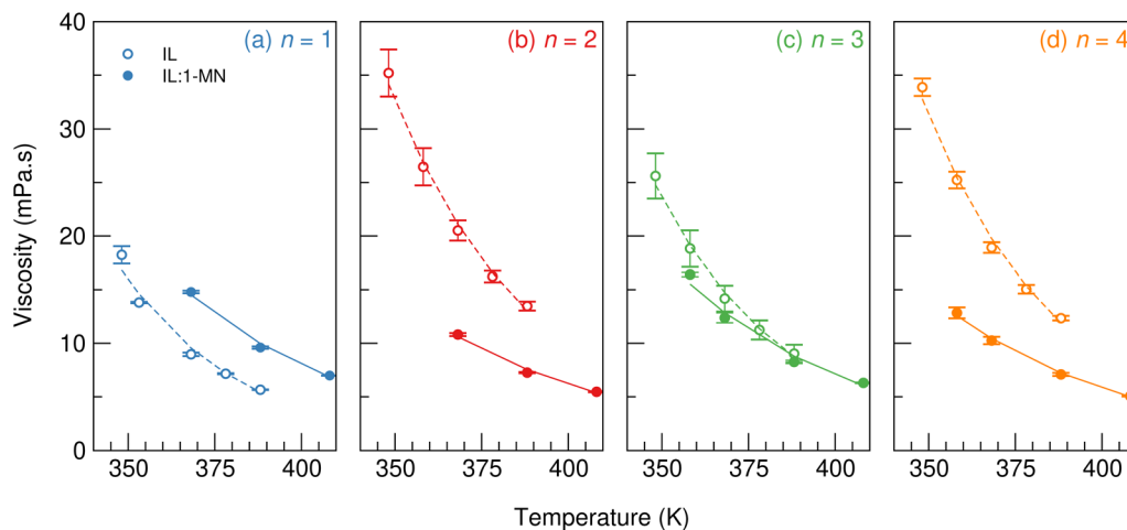
Fig. 5 Plots illustrating the different changes in viscosity upon addition of 1-MN to produce 1 : 1 CT complexes with (a) [C_1^4\text{CNPyl}][\text{NTf}_2] , (b) [C_2^4\text{CNPyl}][\text{NTf}_2] , (c) [C_3^4\text{CNPyl}][\text{NTf}_2] , (d) [C_4^4\text{CNPyl}][\text{NTf}_2] showing the convergence in the viscosities of all four IL : 1-MN CT complexes and the opposite effects on the viscosity between n = 1 with an increase in viscosity and n = 4 with an expected decrease in viscosity on addition of the aromatic diluent.
