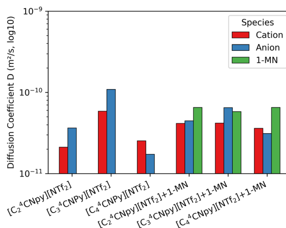
Fig. 14 Diffusion coefficients of the [\text{C}_n^4\text{CNPy}]^+ ( n = 2\text{--}4 ) cations [\text{NTf}_2]^- anions and 1-MN at 60 °C determined from ^1\text{H} and ^{19}\text{F} DOSY NMR spectroscopy on the neat ILs and IL : 1-MN mixtures.
