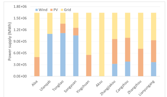
Fig. 7 Energy breakdown of hydrogen production
