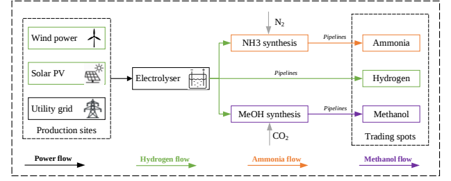
Fig. 1 System configuration
