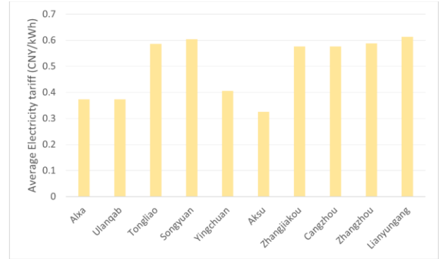
Fig. 4 Average electricity tariffs
