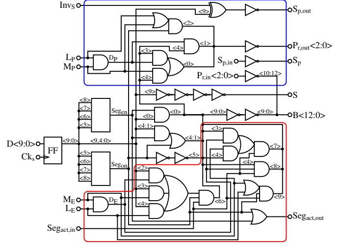
Fig. 3. Schematic of the segment control logic. Gates encircled in red control IQ expansion and gates encircled in blue control phase compensation.
