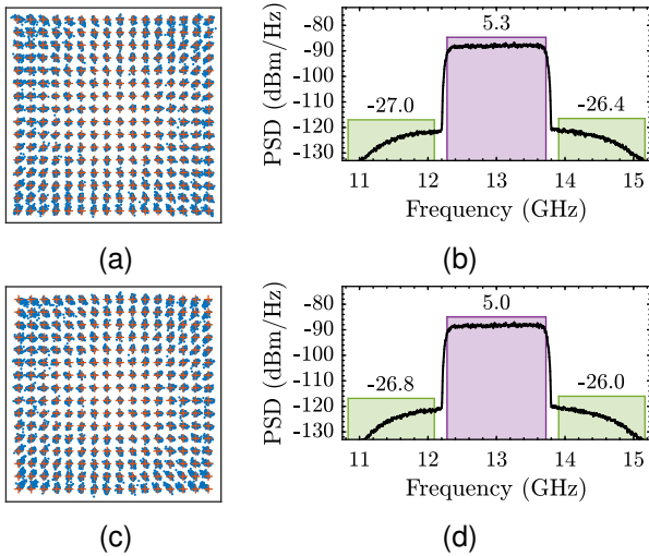
Fig. 8. Constellation diagram and output spectra for 256QAM SC signals using IQ expansion (a) and (b), EVM 2.75 % and ACPR -31.8 dBc, and without using IQ expansion (c) and (d), EVM 3.12 % and ACPR -31 dBc. Both use a sample rate of 6.5 GS/s, achieving a data rate of 17.3 Gb/s with a BER < 10^{-3} . Channel power reported in dBm.
