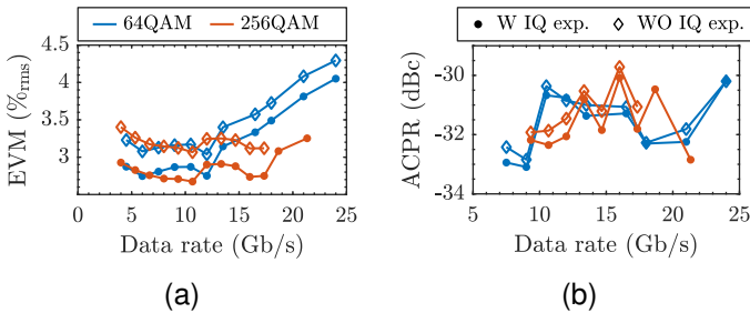
Fig. 6. (a) EVM and (b) ACPR across data rate for 64QAM and 256-QAM SC signals.
