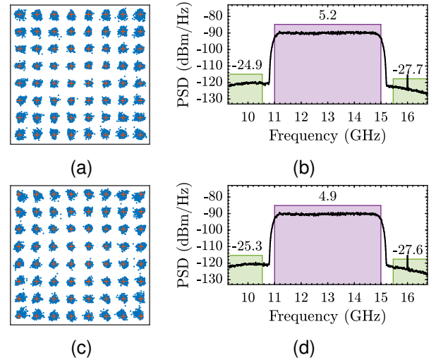
Fig. 7. Constellation diagram and output spectra for 64QAM SC signals using IQ expansion (a) and (b), EVM 4.05 % and ACPR -30.1 dBc, and without using IQ expansion (c) and (d), EVM 4.29 % and ACPR -30.2 dBc. Both use a sample rate of 8 GS/s, achieving a data rate of 24 Gb/s with a BER <10 -4 . Channel power reported in dBm.
