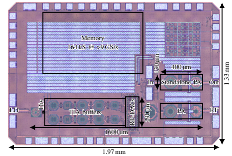
Fig. 4. Chip photo showing the complete transmitter, the standalone PA and the waveform memory.
