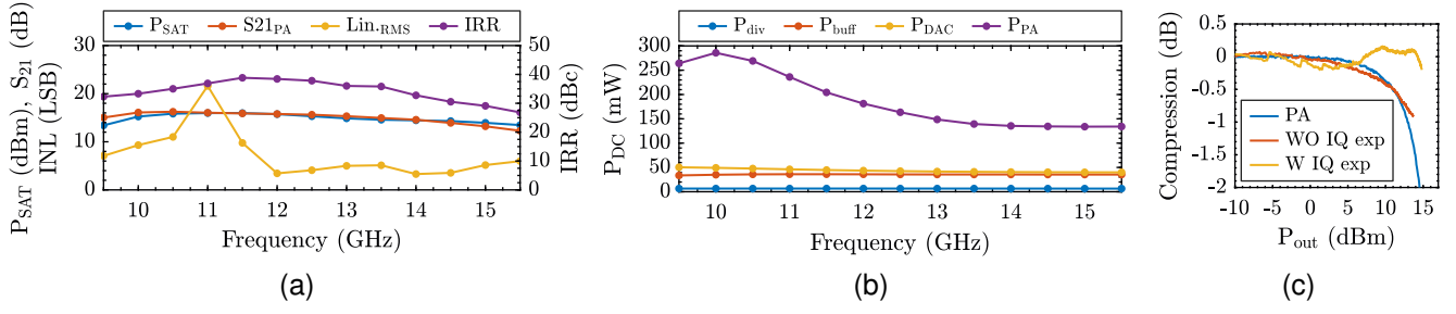
Fig. 5. (a) Saturated RF output power, PA small-signal gain, image-rejection ratio, and integral non-linearity versus carrier frequency. (b) DC power consumption for the divider, TIA buffers, RF-DACs (excluding digital circuits), and PA versus carrier frequency. (c) Compression versus output power for the standalone PA (including attenuator), and for the transmitter with and without IQ expansion enabled. RF-DACs are simultaneously fed with identical input codes.
