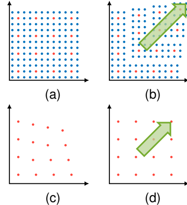
Fig. 1. Cartesian modulator output amplitude/phase combinations for single quadrant using (a) conventional modulator (b) modulator with IQ expansion. (c) and (d) Resulting partial constellation at the PA output when using each respective modulator. These points represent the red points in (a) and (b).
