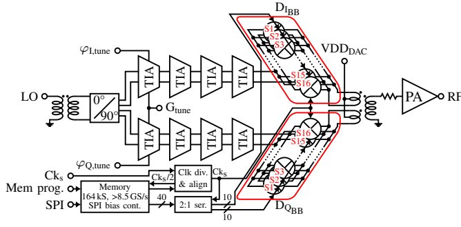
Fig. 2. Transmitter block diagram showing the realization of the complete RF path. RF-DACs are encircled in red.
