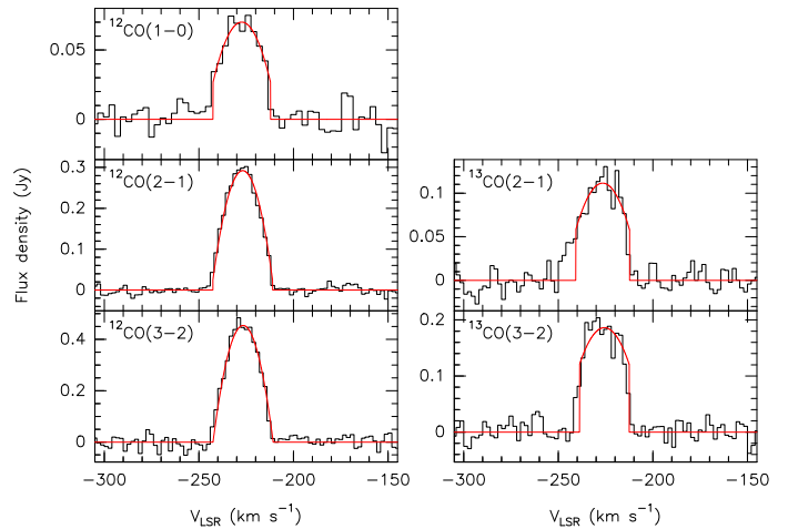
Fig. 6. Spectra of ^{12}\text{CO} 1–0, 2–1, and 3–2, and ^{13}\text{CO} 2–1 and 3–2 towards OH358.052+1.304 (black histogram) and the best shell-line-profile fits (Eq. (3), red solid line) with line-shape parameters H = -0.62, -0.92, -1.0, -0.48 , and -0.35 , respectively. The 1'' data were used. This is an average object in our sample in terms of CO line intensity strengths.
