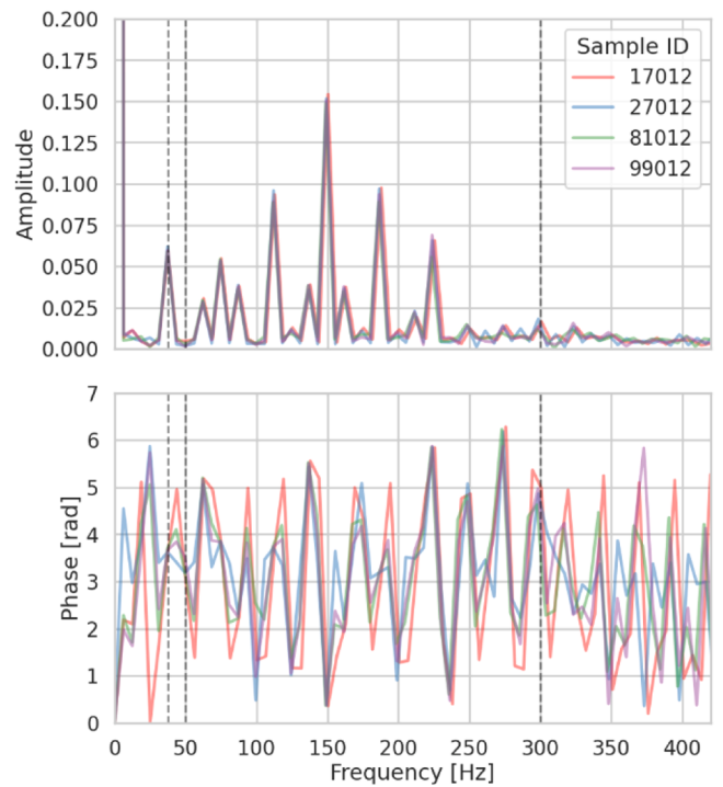
Fig. 14. Fourier transform of four samples as in Fig. 3. HVO100 was used for samples with ID 17,012 and 27,012, and EN590 was used for samples with ID 81,012 and 99,012. The vertical lines highlight 37.5, 50 and 300 Hz, which correspond to the 6th, 8th and 48th Fourier coefficients, respectively.
