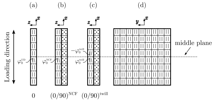
Fig. 13. Initial fibre orientation using the present CDM model. (a) Side view of a 0 UD ply, (b) side view of a [0/90] NCF ply, (c) side view of a [0/90] twill ply, (d) top view of any 0 degree ply.
