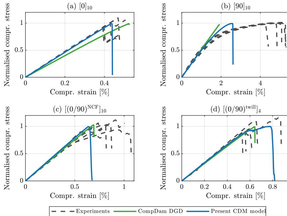
Fig. 15. Experimental and finite element simulation results of compression tests performed on UD, NCF and twill laminates. (a) Longitudinal compression test of UD laminate, (b) transverse compression test of UD laminate, (c)–(d) compression tests of NCF and twill laminates.
