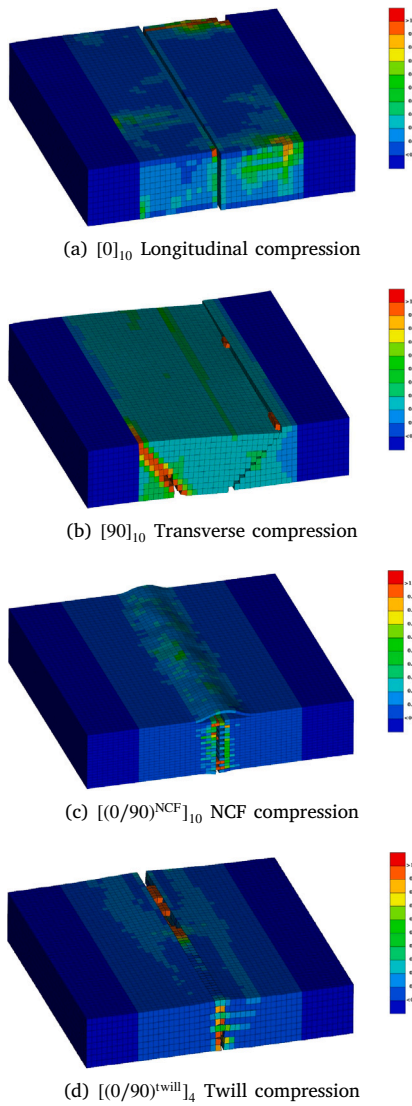
Fig. 16. Based on the calibrated present CDM model, localised deformation patterns obtained from FE simulations of the laminates used for calibration. The images are coloured by the damage variable.
