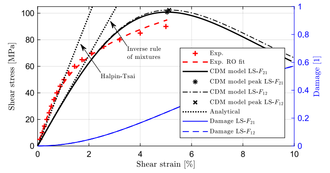
Fig. 6. Experimental and calibrated model shear responses, Ramberg–Osgood curve fitted to experimental data, and analytical initial shear modulus predictions. The experimental data are from the WWFE-III. The last experimental data point corresponds to the in-plane shear strength.
