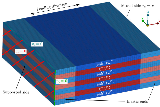
Fig. 12. Finite element mesh and boundary conditions of Laminate A — 0^\circ .
