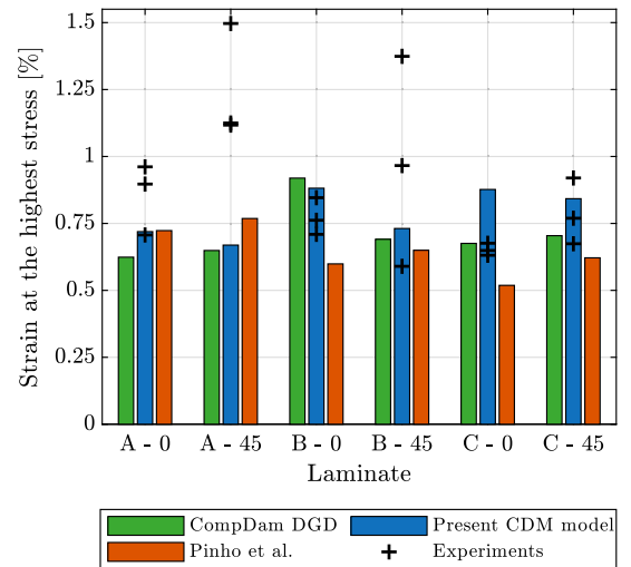
Fig. 20. Strain at the highest stress — experimental and predicted by the model for the different laminates.
