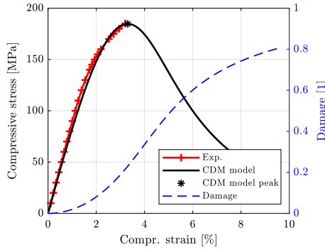
Fig. 4. Experimental and calibrated model response for uniaxial transverse compression. The experimental data are from the WWFE-III.
