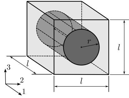
Fig. 3. A representative volume element (RVE) of the microstructure of an undeformed UD ply.
