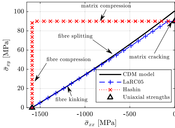
Fig. 9. Maximum stress envelope under combined longitudinal compression and in-plane shear in comparison with failure envelopes of analytical failure models.
