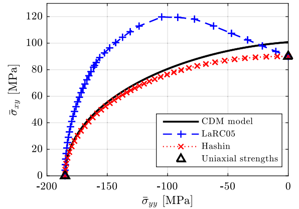
Fig. 10. Maximum stress envelope under combined in-plane transverse compression and in-plane shear in comparison with failure envelopes of analytical failure models.
