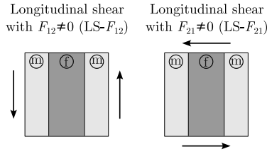
Fig. 5. Schematic representation of the prescribed deformation components used to obtain a pure shear Cauchy stress. The arrows show the direction of prescribed nonzero shear component in the deformation gradient, meanwhile the perpendicular shear is zero. \textcircled{f} — fibre, \textcircled{m} — matrix.
