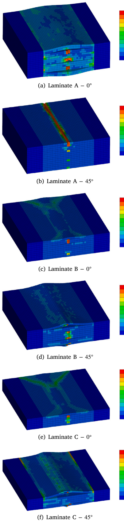
Fig. 18. Deformation patterns of Laminates A, B and C in the validation simulations using the present CDM model. The images are coloured by the damage variable.
