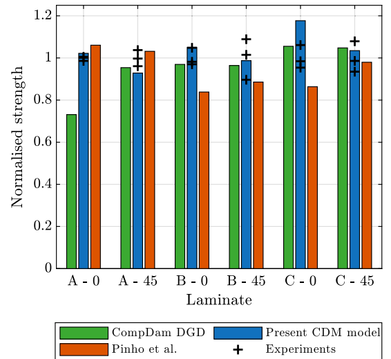
Fig. 19. Experimental and predicted compressive strengths by the model for the different laminates.
