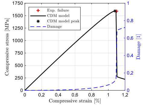
Fig. 7. Experimental and calibrated model response for uniaxial longitudinal compression with an in-plane misalignment angle of \varphi_0 = 1.314^\circ . The experimental data are from the WWFE-III. The longitudinal strain is calculated as \bar{F}_{xx} - 1 .
