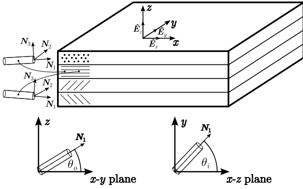
Fig. 2. Definition of the local and global coordinate systems and in-plane and out-of-plane fibre angles.
