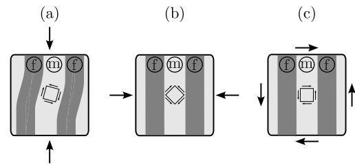
Fig. 1. Planes of maximum shear in the matrix in (a) longitudinal compression in the presence of initial imperfections, (b) transverse compression, and (c) in-plane shear. textcircledf — fibre, m — matrix.
