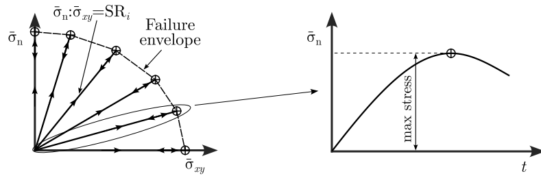
Fig. 8. The procedure of generating failure envelopes with the model presented. (a) Biaxial failure data points and interpolation, (b) maximum stress detection for a given stress ratio.
