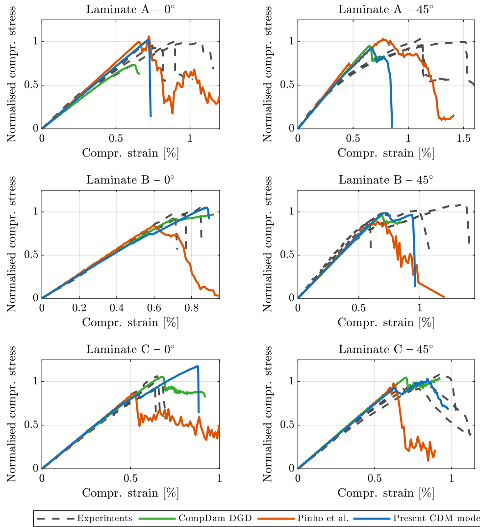
Fig. 17. Experimental and finite element simulation results of compression tests performed on Laminate A, B, and C in 0° and 45° orientations.
