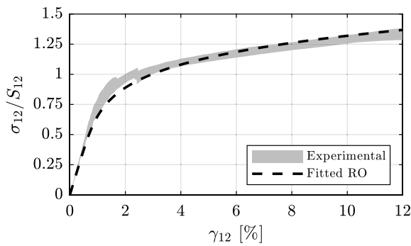
Fig. 14. Range of experimental shear curves and fitted Ramberg–Osgood curve.
