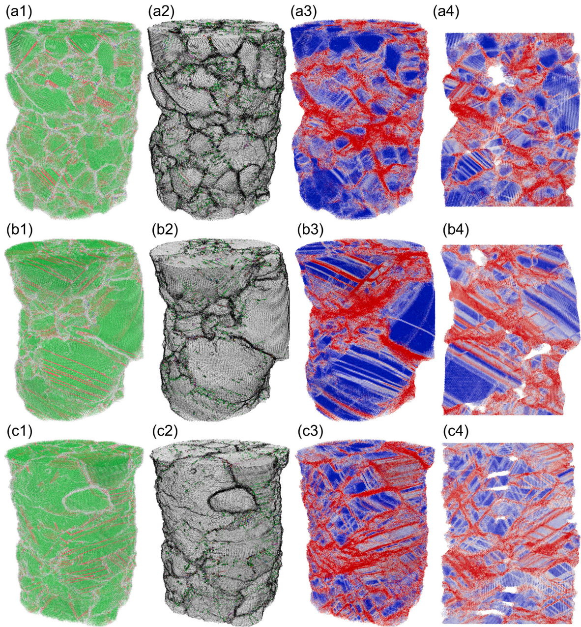
Fig. 8. Post-compression MD simulation results linking particle morphology to dislocation activity and local strain distribution in sintered Cu pillars. (a1–a4) Atomic structure, dislocation distribution, atomic strain distribution, and corresponding cross-sectional strain map of the monomodal structure. (b1–b4) Corresponding results for the bimodal structure. (c1–c4) Corresponding results for the flake-shaped structure.
