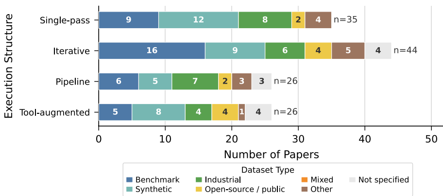
Fig. 48 Dataset types used for evaluation by execution structure (RQ2 \times RQ4)
