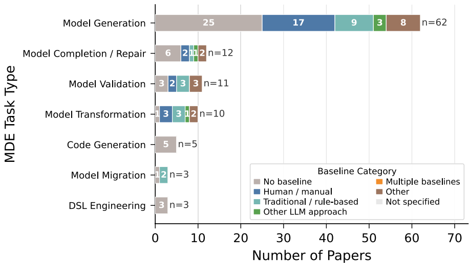
Fig. 46 Baseline comparison categories by MDE task type (RQ1 × RQ4)
