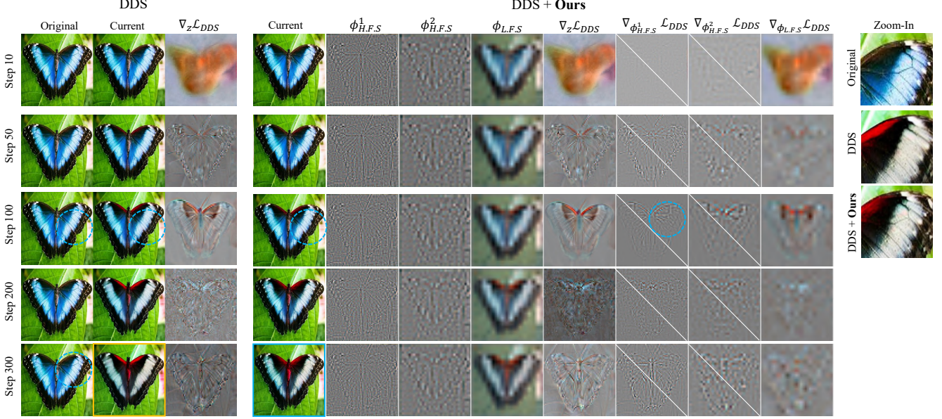
Figure 6. Gradient visualization during optimization. Edit with “A photo of a (blue → red) butterfly”. We visualize the frequency-decomposed representation \phi (with three subbands, \phi_{H.F.S.}^1 , \phi_{H.F.S.}^2 and \phi_{L.F.S.} ), the gradients at the latent level \nabla_z \mathcal{L}_{DDS} , as well as gradients at subband level \nabla_{\phi} \mathcal{L}_{DDS} in multiple wavelet subbands. As shown, although the optimization points towards the target, the gradients at each step exhibit randomness ( \nabla_z \mathcal{L}_{DDS} in step 50 and step 100). This is due to the noise added during the sampling procedure and tends to smooth out or distort detail patterns. With our method, we apply a stop-gradient operator to preserve these details (right). Note that we add a diagonal line to indicate the subband gradients where the stop-gradient operator is applied. Best viewed on a screen when zoomed in.
