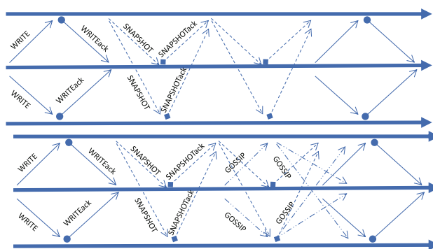
Fig. 1. Examples of Algorithm 1’s executions. The upper drawing illustrates a case of a terminating snapshot operation (dashed line arrows) that occurs between two write operations (solid line arrows). The acknowledgments of these messages are arrows that start with circles and squares, respectively. The lower drawing depicts the execution of Algorithm 1’s self-stabilizing version for the same case illustrated in the upper drawing. Note that the gossip messages do not interfere with other messages.
