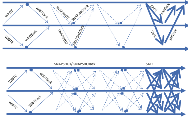
Fig. 3. The upper drawing depicts an example of Algorithm 3's execution for a case that is equivalent to the one depicted in the upper drawing of Fig. 2, i.e. , only one snapshot operation. The lower drawing illustrates the case of concurrent invocations of snapshot operations by all nodes.
