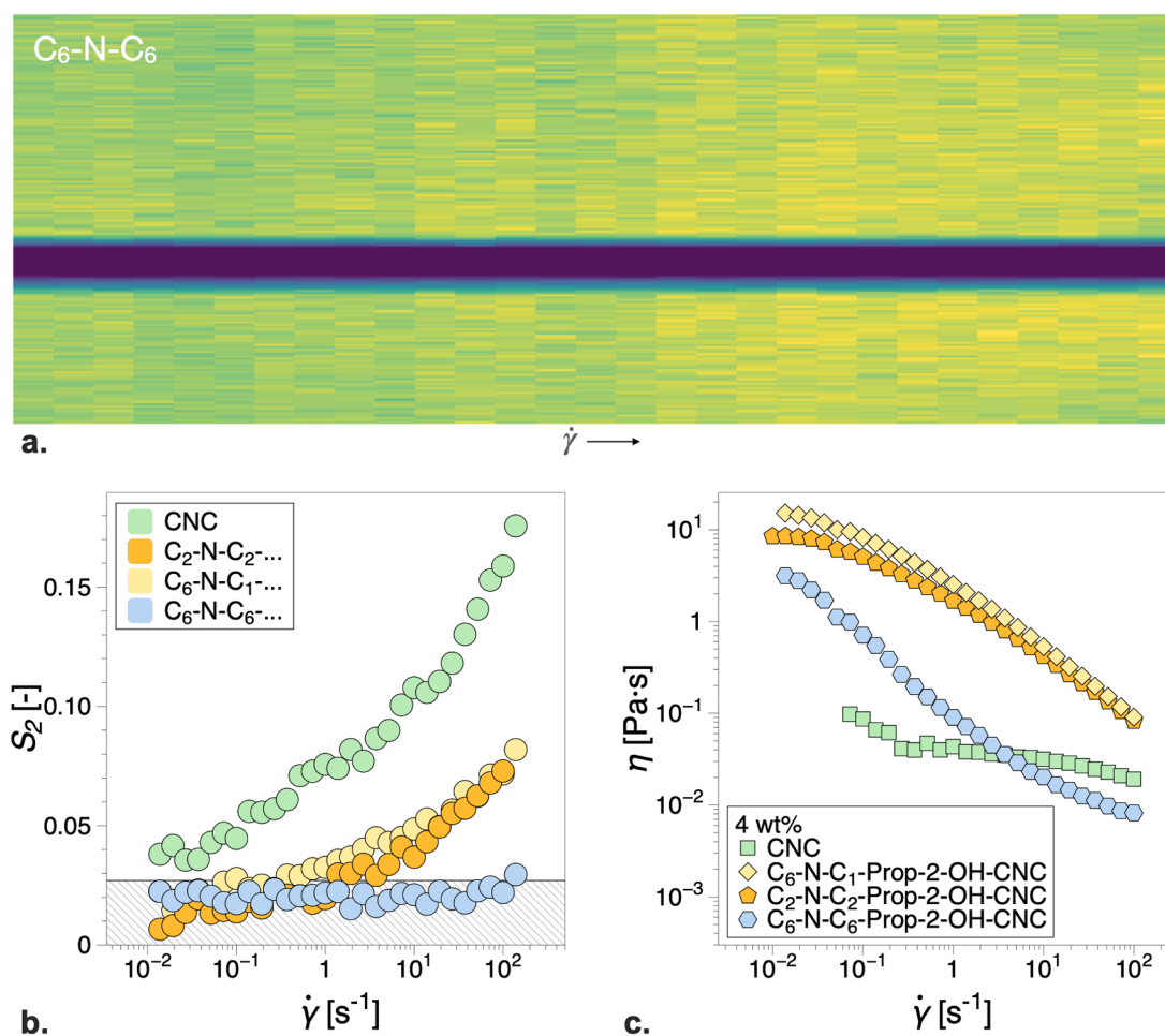
Fig. A.7. (a) Azimuthal integration data corresponding to C_6-N-C_6 showing the absence of a reliably identifiable anisotropy peak. (b) Hermans anisotropy parameter, S_2 , and (c) shear viscosity functions for the data in Fig. 3.
