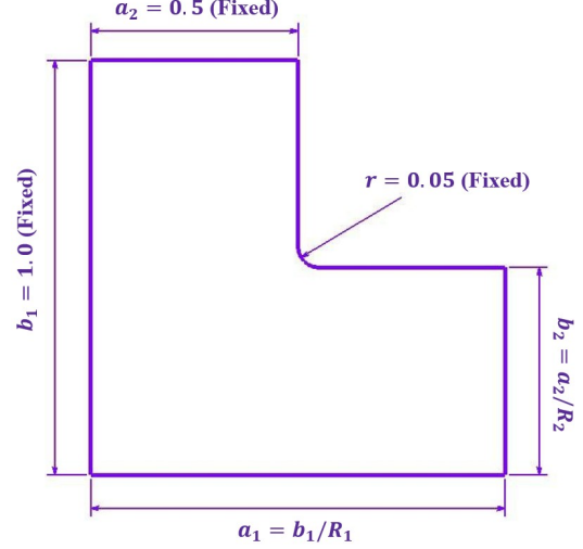
Figure 1: Parametric L-shaped slab geometry
