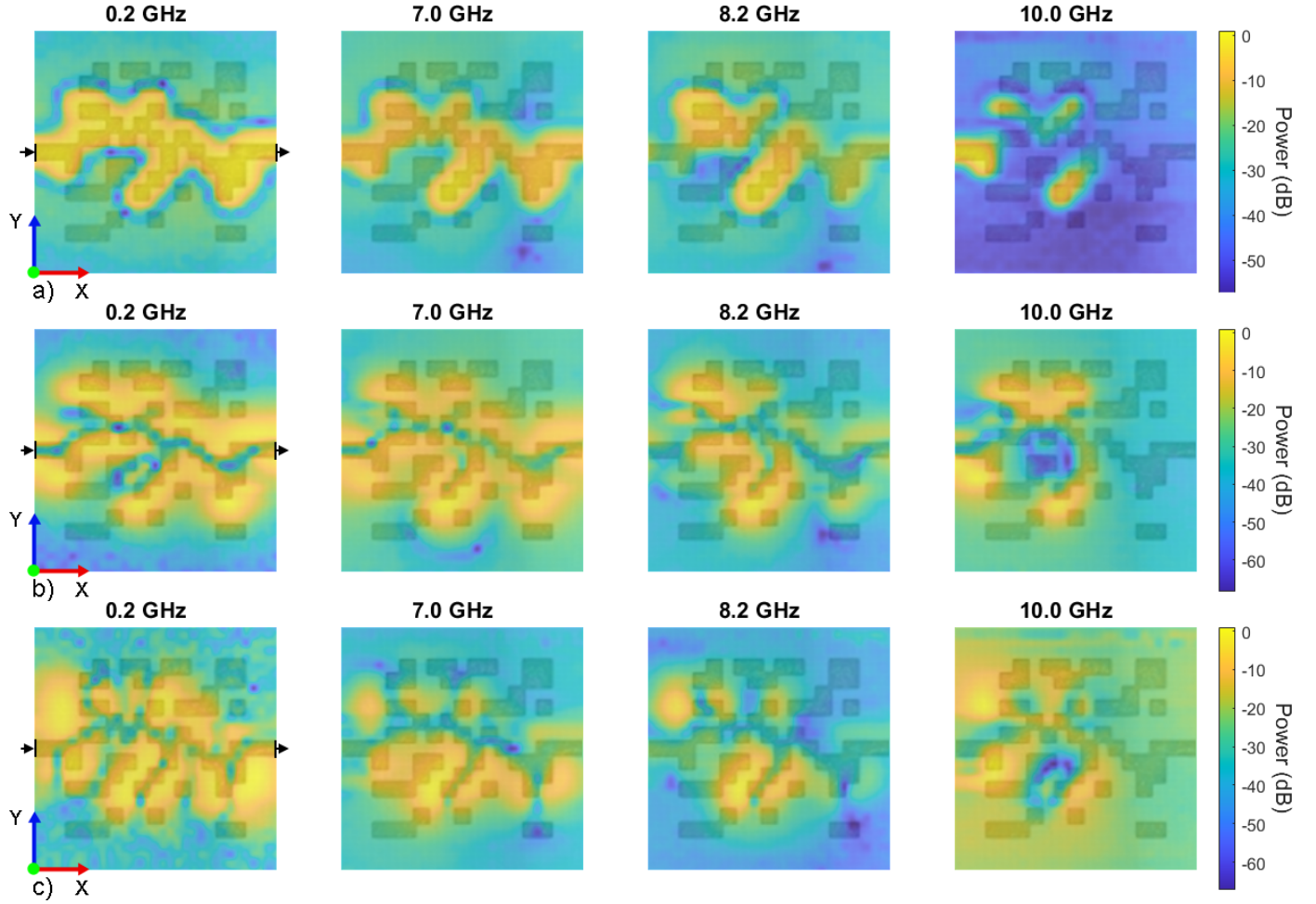
Fig. 4. Normalized measured (a) E_Z , (b) E_Y and (c) E_X from S_{21}^{EO} in dB mapped over a photo (dimension: 15.3×15.3 mm) of the filter for four frequencies. The input and output are indicated with black arrows. The data is normalized at each frequency to maximize contrast. The orientation of x and y is indicated in the left figures.
