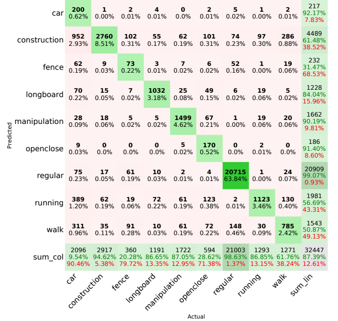
Fig. 3. Confusion matrix for the test set using the CNN with architecture inspired by [6]. Note the near-perfect recall on the dominant regular class (>98%) contrasted with poor recall on minority classes: car achieves only ~10% recall with most samples misclassified as construction .
