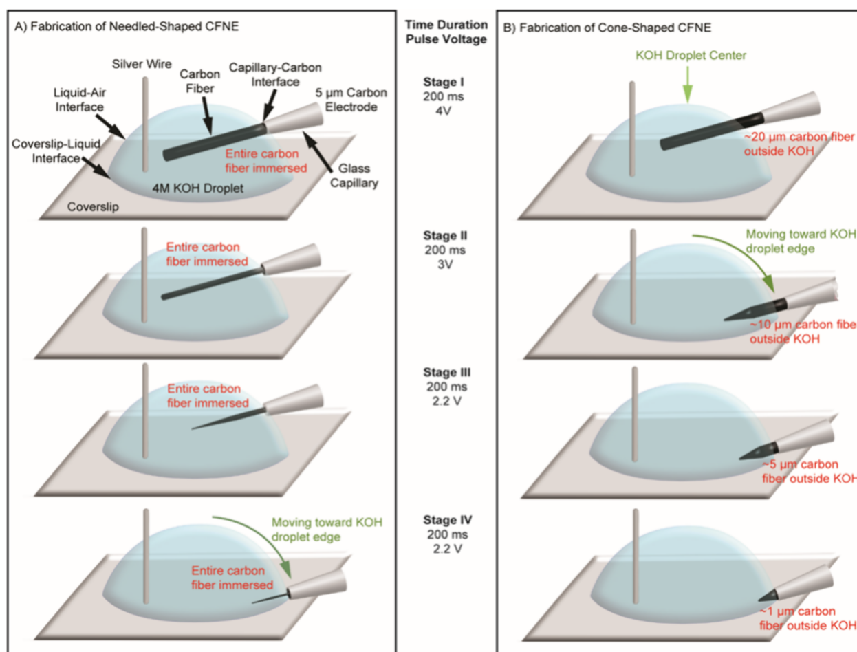
Figure 3. Stepwise electrochemical droplet etching strategy for fabricating CFNEs with distinct geometries. Schematics illustrate the fabrication of (A) needle-shaped (left) and (B) cone-shaped (right) CFNEs using a stepwise etching process. This method relies on applying 200 ms voltage-controlled pulses combined with precise micromanipulation of the electrode position and depth of carbon fiber immersed in a KOH droplet. These parameters are critical for shaping the final geometry of the nanotip. Initially (Stage I), the CFME is positioned at the center-top of the droplet. During the etching process, the electrode tip is gradually lowered toward the edge of the KOH droplet near the microscope coverslip-liquid interface (Stages II–IV). (A) To create needle-shaped tips, the entire cylindrical carbon fiber is fully submerged into the droplet, aligning the glass capillary-carbon fiber interface with the droplet’s liquid-air surface. (B) In contrast, cone-shaped electrode tips are produced by partially submersing the carbon fiber tip into the droplet while keeping a portion of carbon fiber (20 \mu\text{m} to 1 \mu\text{m} ) outside the KOH droplet, thereby selectively etching the exposed portion of the fiber. Schematics are not drawn to scale.
