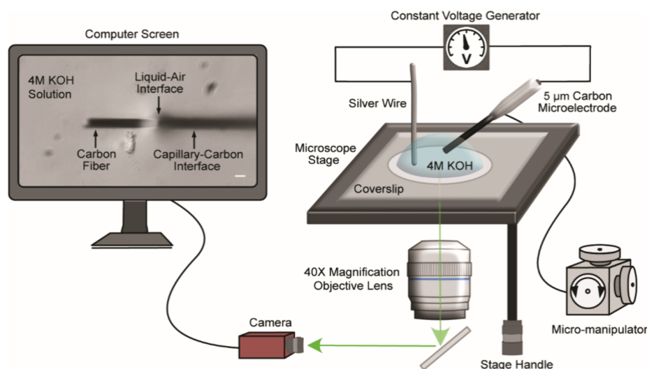
Figure 1. Experimental setup for gentle, stepwise electrochemical etching of carbon fiber nanotip electrodes (CFNEs) with real-time microscopy imaging and camera projection onto a computer screen. A standard hemocytometer was used to create a calibrated ruler on the computer screen. The movable microscope stage and a micromanipulator are used to adjust the placement of the carbon fiber microelectrode (CFME) tips at the liquid-air interface of a 4 M potassium hydroxide (KOH) droplet serving as the etching solution. A voltage pulse generator (Digitimer DS2A-Mk.II) was used to apply time- and amplitude-controlled voltage pulses to the electrode surface versus a silver electrode. The white scale bar on the computer screen (left) is 5 \mu\text{m} . Schematics are not drawn to scale.
