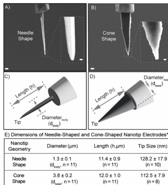
Figure 4. Scanning electron microscopy images of representative (A) needle-shaped and (B) cone-shaped carbon fiber nanotip electrodes (CFNEs) with tip diameters of approximately 100 nm. The scale bars in panels (A) and (B) indicate 1 \mu\text{m} , with additional scale bars of 100 nm shown in the inset images. (C) and (D) illustrate the defined measured dimensions of needle-shaped and cone-shaped CFNEs, respectively. (E) Table summarizing the measured dimensions of needle-shaped and cone-shaped CFNEs as determined by scanning electron microscopy image analysis of the differently shaped CFNEs, reported as mean \pm SEM, unless otherwise indicated. While (C) and (D) show idealized axisymmetric schematics to define dimensional parameters, the images in (A) and (B) reflect the physical reality of fabricated CFNEs, which may exhibit minor geometric asymmetries. These result from droplet curvature, variable immersion depth at the droplet edge, and limitations of manual alignment during the fine-tuning of the electrode geometry.
