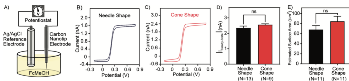
Figure 5. Electrochemical characterization of CFNEs using cyclic voltammetry. (A) Schematic illustration of the experimental setup for cyclic voltammetry (not drawn to scale). Representative cyclic voltammograms of (B) a needle-shaped CFNE (black) and (C) a cone-shaped CFNE (red), recorded in 1 mM ferrocenemethanol (FcMeOH) solution. (D) Comparison of steady-state current amplitude at +0.6 V for needle-shaped ( n = 13 , black) and cone-shaped ( n = 9 , red) CFNEs. (E) Surface area estimates for needle-shaped ( n = 11 ) and cone-shaped ( n = 11 ) CFNEs based on SEM analysis. In (D) and (E), data are displayed as the mean \pm SEM. The Mann-Whitney (two-tailed, unpaired) test was performed for statistical comparison, with “ns” indicating no significant difference.
