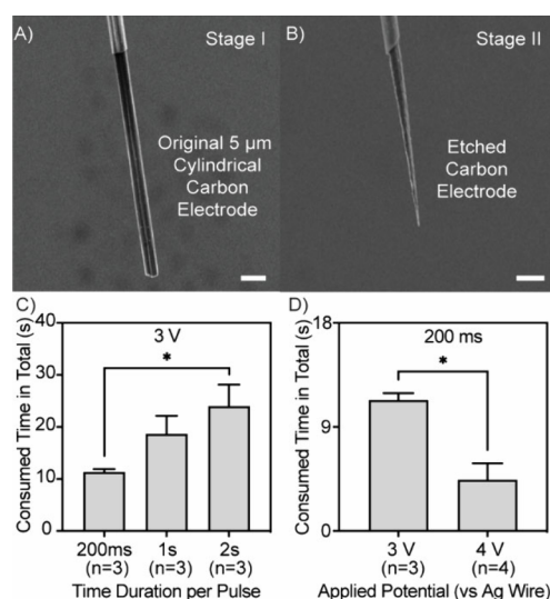
Figure 2. Scanning electron microscopy images of (A) a representative 50 \mu\text{m} long, 5 \mu\text{m} cylindrical carbon fiber microelectrode (CFME) before etching (Stage I) and (B) a 30 \mu\text{m} long cone-shaped carbon fiber nanotip electrode (CFNE) (Stage II) produced after KOH droplet etching. Scale bars in parts (A) and (B) represent 10 \mu\text{m} . (C, D) Analysis of etching efficiency and total etching time during the etching of a cylindrical CFME into a cone-shaped nanotip electrode. In (C), etching time was evaluated by varying pulse durations (200 ms, 1 s, and 2 s) while applying 3 V pulses. In (D), etching time was assessed by varying the applied potential (3 and 4 V) while keeping the pulse duration constant at 200 ms. Data are presented as the mean \pm the standard error of the mean (SEM). A two-tailed unpaired t -test was performed for comparison, *p < 0.05 .
