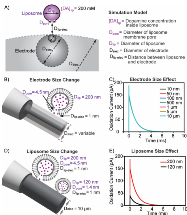
Figure 8. Prediction of amperometric DA detection efficiency as a function of electrode dimensions, liposome size, and spatial parameters relevant to the experimental amperometric recording of liposome rupture events. (A) Schematic of the simulation model used to evaluate DA detection efficiency by CFNEs from single liposomes, considering variation in electrode and liposome size, where the model computes DA release from an initial membrane pore, followed by the diffusion of DA through the pore, and subsequent diffusive flux to the electrode surface. (B) Illustration of the simulation framework used to assess how the CFNE diameter influences DA detection efficiency. (C) Simulated amperometric traces of DA release from a 4.5 nm membrane pore of a 200 nm liposome recorded using cylindrical electrodes with varying diameters (10 nm to 10\ \mu\text{m} ), showing how electrode size influences current spike shape and amplitude. Although seven conditions were simulated, the curves nearly completely overlap due to the minimal effect of electrode diameter under this configuration. (D) Schematic of the model used to evaluate the impact of liposome size on DA detection efficiency. (E) Simulated amperometric traces showing DA release from liposomes of two sizes, 200 nm (4.5 nm pore) and 120 nm (1.4 nm pore), interacting with a 10\ \mu\text{m} cylindrical electrode, assuming a 1 nm liposome-electrode distance. All simulations assume a DA diffusion coefficient of 6 \times 10^{-10}\ \text{m}^2\ \text{s}^{-1} . Schematics are illustrative and are not drawn to scale.
