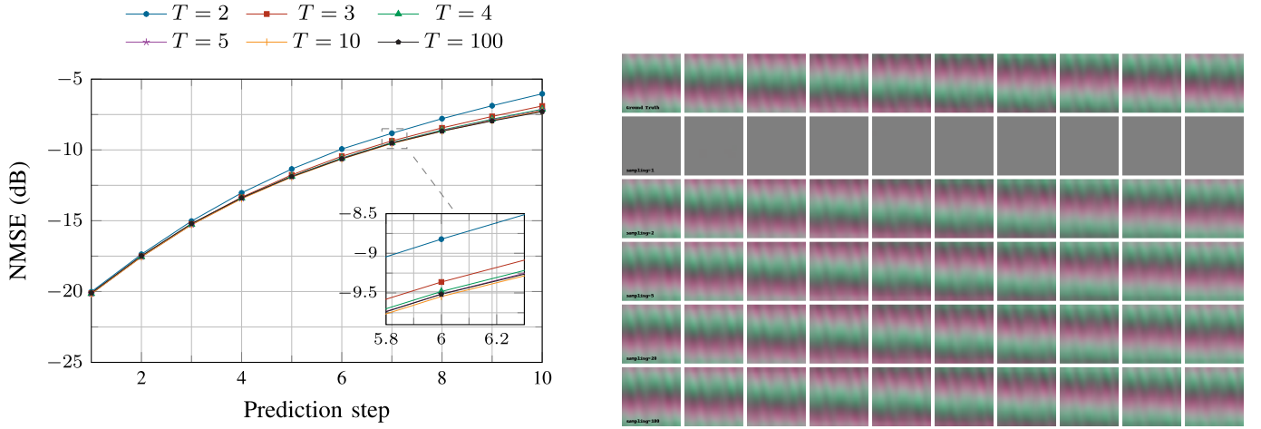
Fig. 7. Left: NMSE performance versus prediction step at 10 dB SNR for different sampling steps. Right: qualitative channel visualization for a single sequence, where rows correspond to the ground truth and predictions for each sampling step, and columns indicate the prediction steps.
