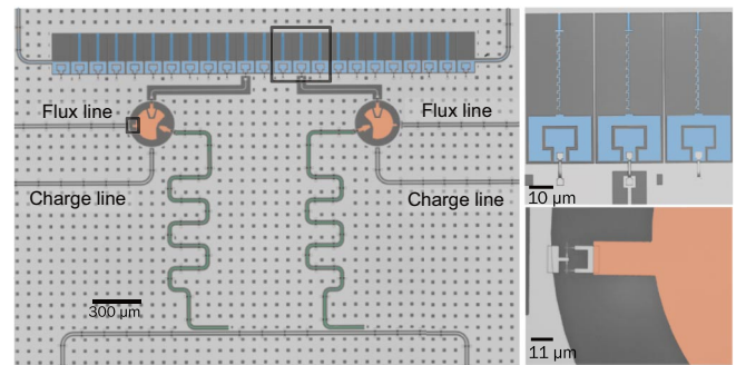
FIG. 6. False-colored image of the device. Connections to the transmon are labeled for clarity. In blue: resonator array, in orange: two transmon qubits, in green: readout resonators for the transmons. Insets outlined in black: top corresponds to a close-up of three resonators with the array of 10 Josephson junctions. Bottom: asymmetric SQUID for the transmon.
