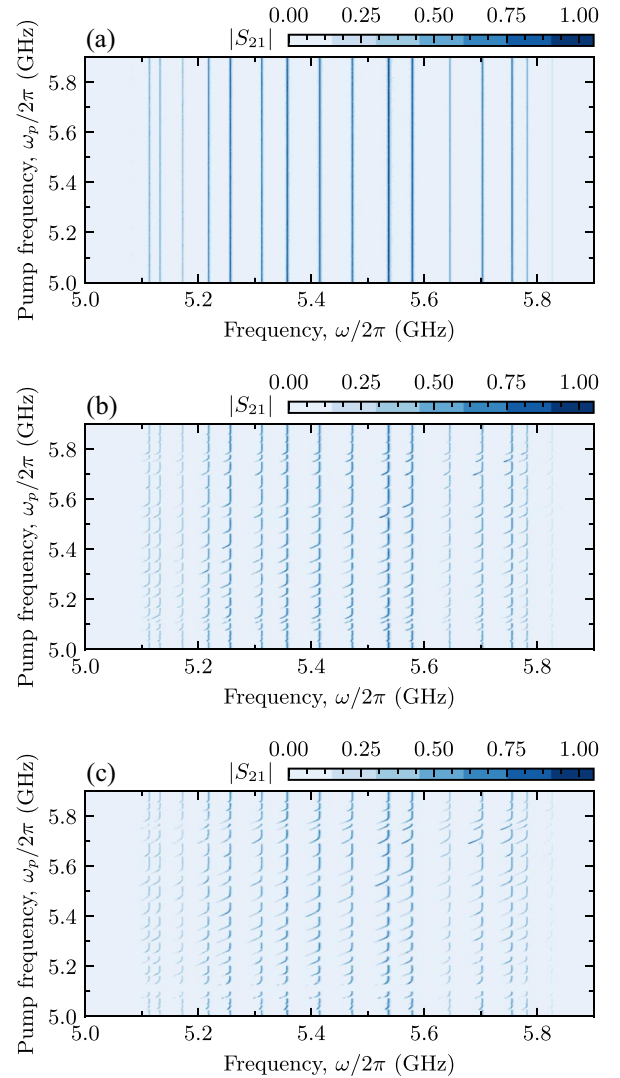
FIG. 7. Transmission band depending on pump frequency and power. (a) Low pump power \epsilon/\gamma = 0.14 . The transmission response is not affected by the pump. (b) At intermediate powers, \epsilon/\gamma = 14.07 , first-order transitions appear, reported in the main text. (c) At high pump power \epsilon/\gamma = 28.08 some modes disappear.
