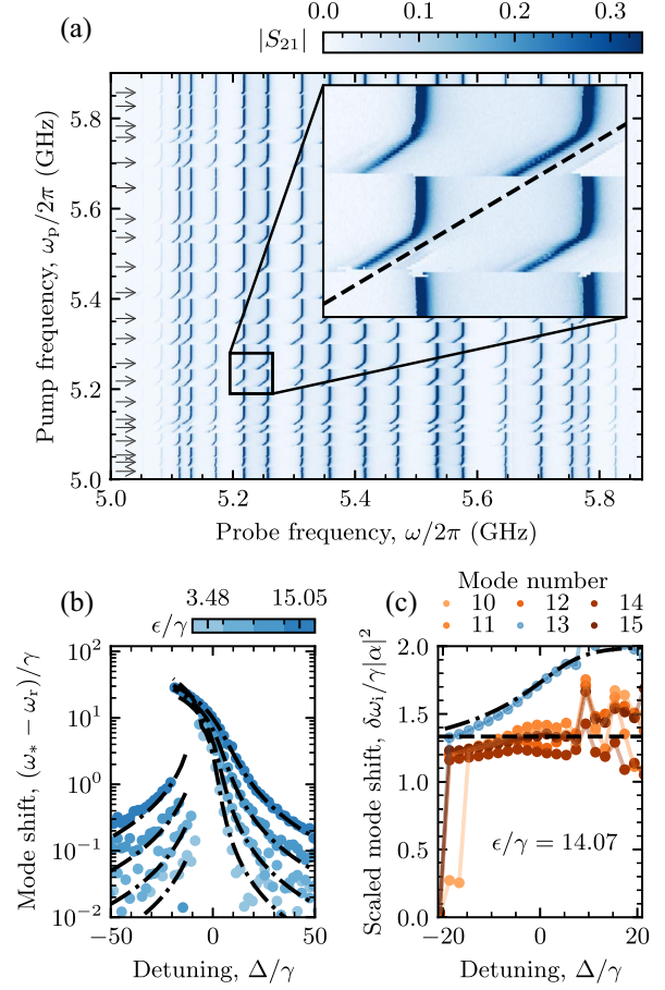
FIG. 2. Spectroscopic evidence of the phase transition. (a) Transmission across the chain, |S_{21}| versus probe and pump frequencies at a fixed pump amplitude \epsilon/\gamma = 14.07 . Each horizontal arrow corresponds to the resonant frequency of a mode of the undriven chain. When the pump is close in frequency to any of the modes (dashed black line in the inset), the resonance frequencies of all modes shift abruptly. (b) Mode-13 frequency shift versus normalized pump detuning, \Delta/\gamma for selected pump amplitudes (color bar). Theory model results from Eqs. (4) and (5) are shown as dash-dotted lines. (c) Normalized frequency shifts of center-band modes (indices 10 to 15), \delta\omega_i/(\gamma|\alpha|^2) versus \Delta/\gamma at fixed pump amplitude. Corresponding theory predictions from cross-Kerr model for non-resonant (resonant) modes are plotted as dashed (dot-dashed) lines.
