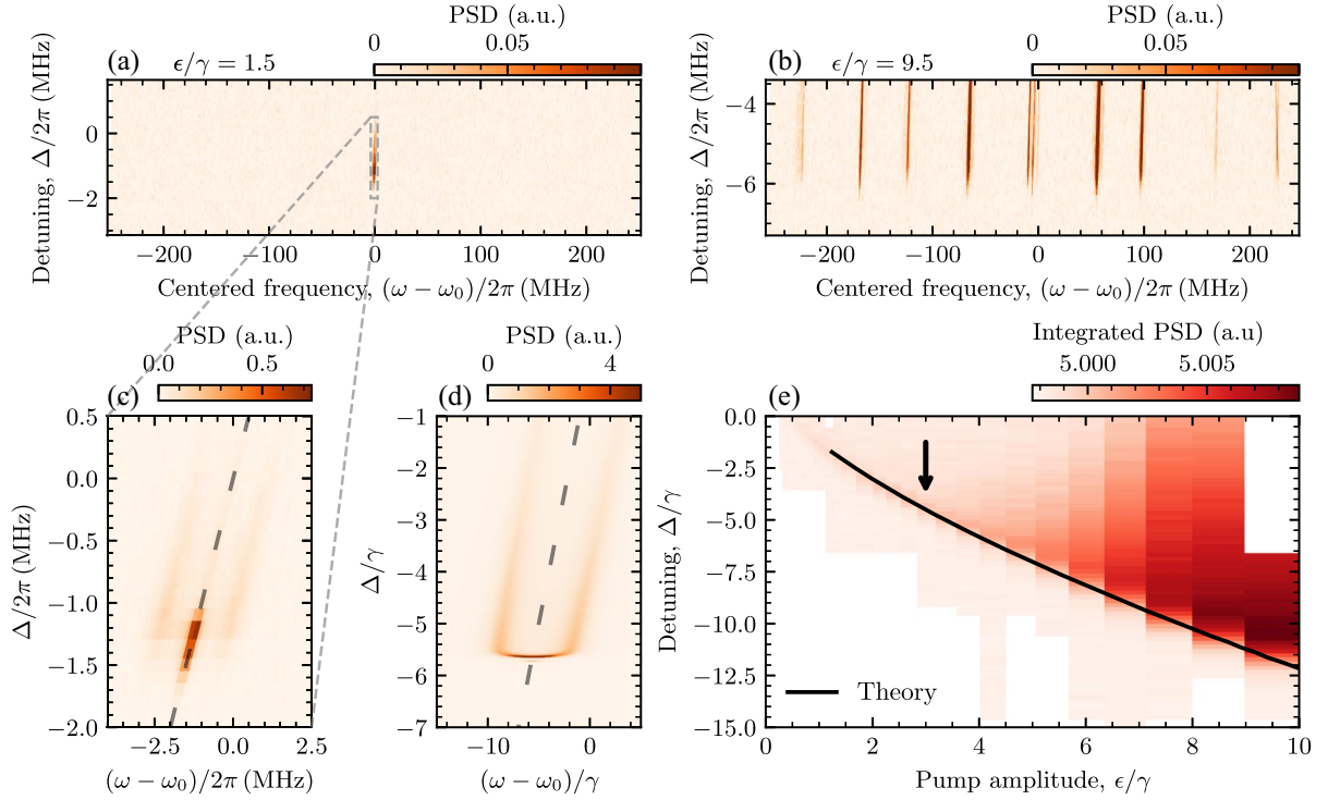
FIG. 3. Photon emission from the metamaterial. (a) PSD against detuning over several modes at moderate pump power \epsilon/\gamma = 1.5 . Only the quasi-resonant mode emits. (b) PSD against detuning over several modes at a larger pump power, \epsilon/\gamma = 9.5 . Other modes of the chain start to emit. (c) Enlarged view of the resonant mode emission spectrum. (d) Theory prediction of the emission spectrum in (c) (note the different scales). (e) Integrated power spectral density against detuning and pump amplitude. High emission indicates a high photon number stored in the mode: we observe a phase boundary between the dim and bright states. The numerically computed transition line is in black. The transition between single-mode and multimode emission is indicated by a black arrow.
