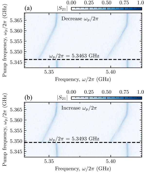
FIG. 8. Hysteresis of the system. (a) The pump frequency is swept decreasingly (high to low). (b) The pump frequency is swept increasingly (low to high).
