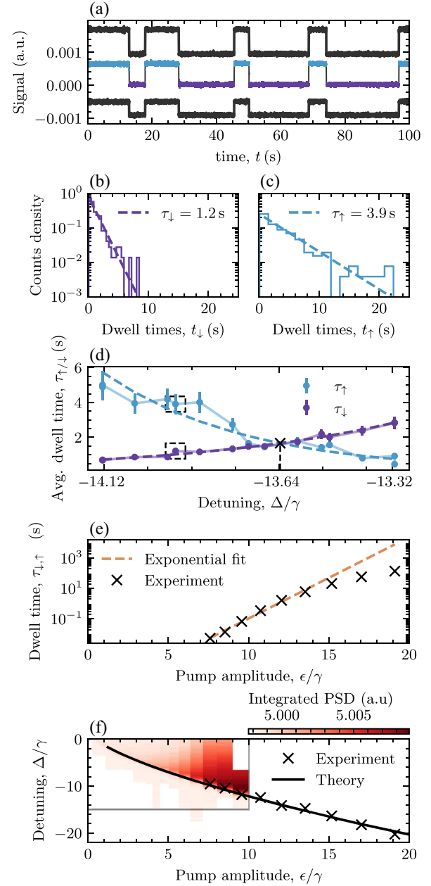
FIG. 4. Time-resolved measurements. (a) Portion of measured time trace for the resonant (color) and adjacent modes (gray). The bright dwell times are in purple, the dim dwell times in blue. (b) and (c) Histograms of dwell times reported for one value of detuning and pump amplitude [Square in (d)]. Estimated exponential density probability functions in dashes, providing the characteristic dwell times. (d) Characteristic dwell times in bright and dim states against detuning at finite pump amplitude. Their intersection provides the transition location. Exponential model fits in dashes. (e) Dwell times at the first-order transition line. Dashed line: exponential fit to the data. (f) Extended phase diagram in the detuning/pump amplitude plane. The integrated PSD data within the gray rectangle is the same as in Fig. 3(e). Crosses denote direct measurements of the first-order transition line obtained by dwell-time measurements as in panel (d). The transition line predicted by theory is shown as a black line.
