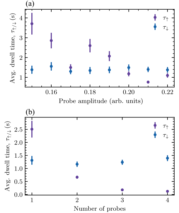
FIG. 9. Effect of the signal probe on the dynamics of the system. (a) Effect of the probe amplitude on the rates. (b) Effect of the number of modes being probed.
