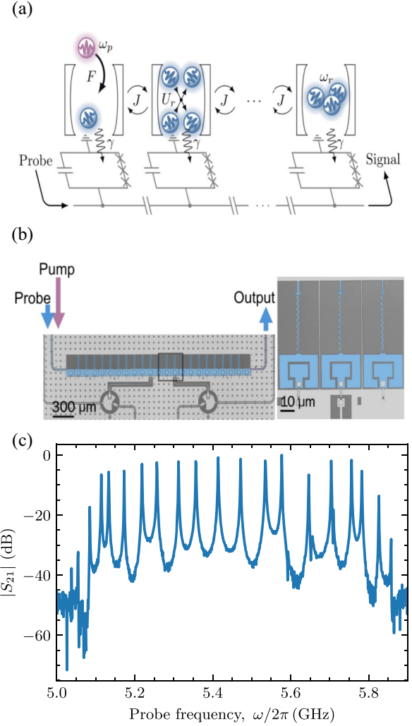
FIG. 1. Bose-Hubbard chain characterization. (a) Schematic representation of our experiment, with N cavities with energy \omega_r , nonlinearity U_r , jumping rate J , and decaying rate \gamma . The circuit diagram with LC resonators capacitively coupled is also included. (b) False-color micrograph of the device, including external connections. Blue: lumped-element resonator array forming the Bose-Hubbard chain. The inset, marked with the black square, shows three resonators with their array of Josephson junctions as the nonlinear inductance. (c) Transmission of the chain as a function of frequency, with the 21 modes of the system showing up as peaks.
