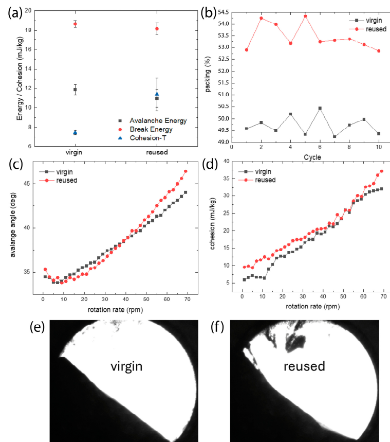
Figure 11. Rheological characterisation of virgin and reused powders: (a) flowability metrics, including avalanche energy, break energy, and cohesion, measured at a constant rotational speed of 0.6 rpm; (b) packing density; (c) avalanche angle; and (d) cohesion. Avalanche morphologies of the (e) virgin and (f) reused powders measured at 1 rpm.
