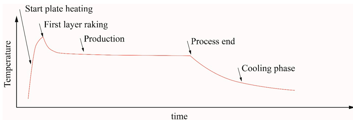
Figure 1. Temperature profile measured by thermocouple, with the principal phases where temperature changes.
