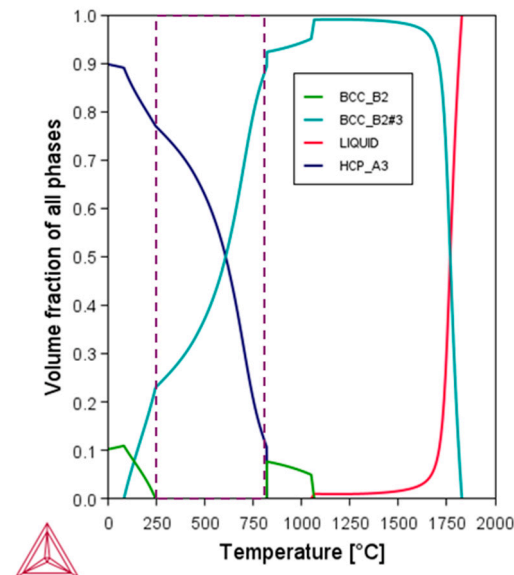
Figure 2. CALPHAD-predicted phase volume fractions as a function of temperature for the Ti21S alloy. In the phase labels, the suffix “#n” identifies compositionally different instances of the same phase.
