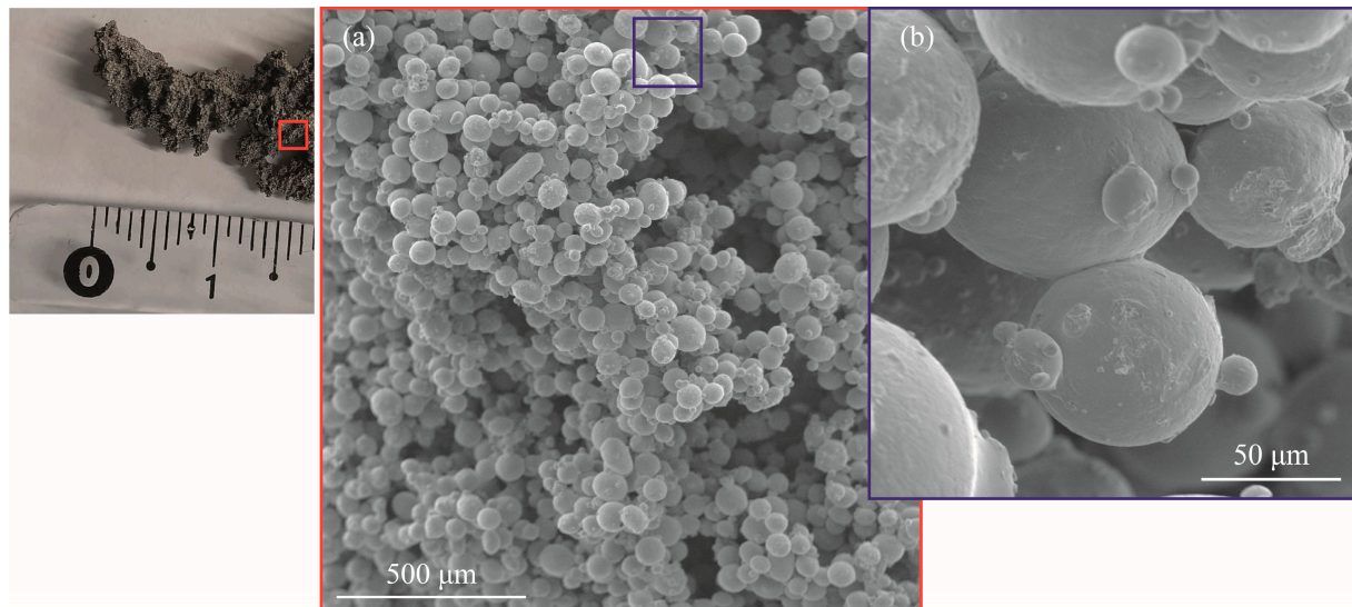
Figure 7. Agglomerated powder structure recovered from the build chamber after the second build: (a) Morphology of powder particles and (b) detail of the necking between two particles.
