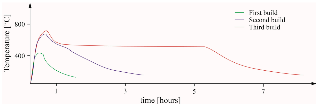
Figure 4. Temperature evolution during the builds measured by the thermocouple positioned under the start plate.
