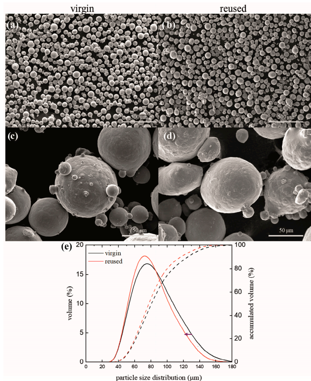
Figure 9. Powder morphology of virgin (a,c) and reused (b,d) powders, and their particle size distribution (e).
