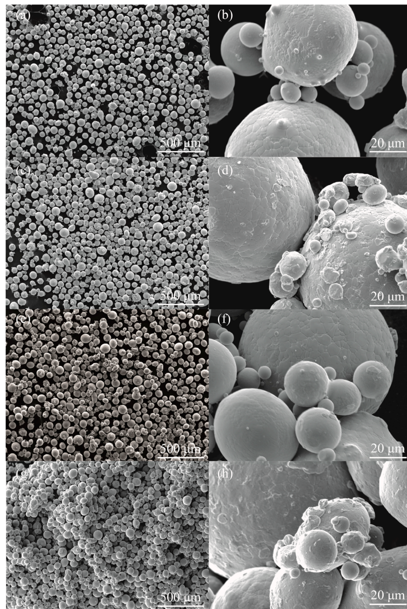
Figure 3. Powder morphology of agglomeration of particles after sintering experiments using TG apparatus at magnifications 100× (a,c,e,g) and 2000× (b,d,f,h), respectively at: 400 °C (a,b), 500 °C (c,d), 600 °C (e,f) and 700 °C (g,h).
