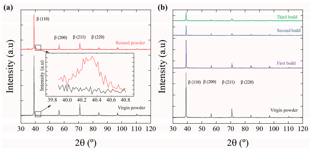
Figure 10. XRD patterns of \beta -Ti21S virgin and reused powder. (a) Comparison between virgin powder and powder reused after the three builds in the PBF-EB. (b) Comparison between the XRD patterns of virgin powder and the pattern for powder extracted after the first, second and third build in the PBF-EB.
