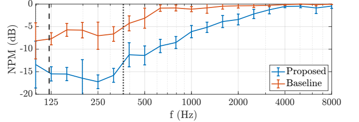
Fig. 4. Mean and standard deviation of binaural NPM based on measurements with a moving microphone array in three different rooms.
