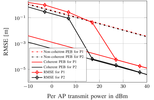
Figure 4: RMSE of the UE position estimate, and PEB for transmission protocols P1 and P2 .
