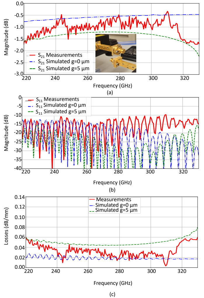
Fig. 7. Comparison between simulated and measured scattering parameters. (a) Transmission parameters. (b) Reflection parameters. (c) Losses of the waveguide channel in dB/mm.
