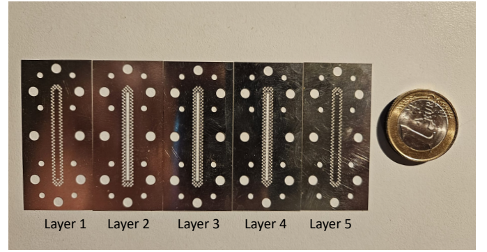
Fig. 6. Manufactured five-layer silver-plated MLW
