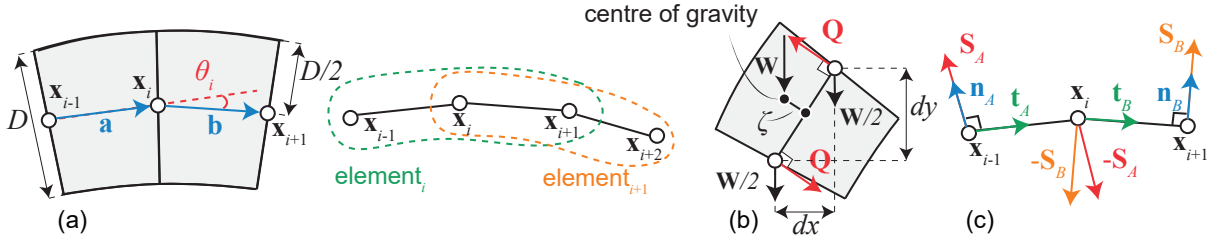
Figure 3: In (a), a discrete model of a quadratic B-spline beam element with three nodes is shown, along with how two neighbouring elements share two of these nodes. In (b), the manner in which the load from a masonry wedge is transferred to the nodes. In (c), the way shear forces from an element are transferred to the nodes.
