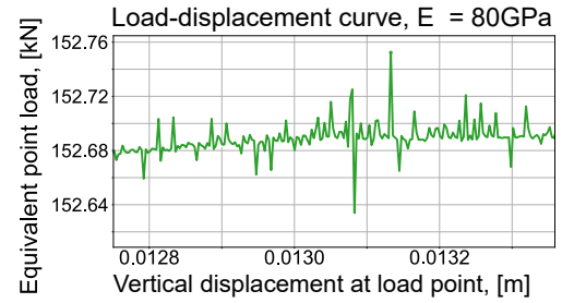
Figure 7: Close-up of the load–displacement curve for E = 80 GPa in Figure 6.
