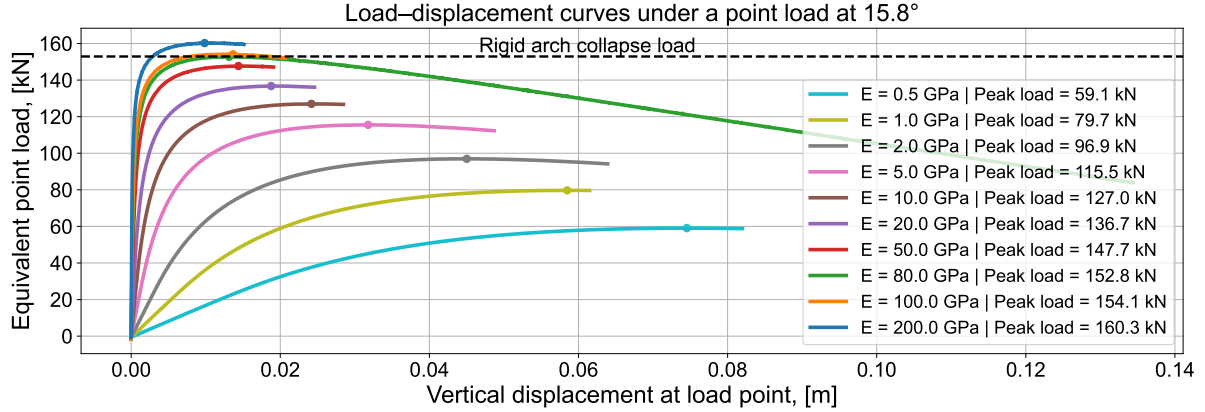
Figure 6: The load–displacement curves for the cracked elastic arch using different Young’s moduli. The dashed horizontal line is the collapse load for the rigid arch. The resolution is illustrated in a magnified section in Figure 7.
