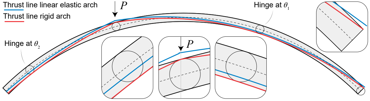
Figure 4: Line of thrust for the rigid arch in red and the linear elastic arch in blue. The circles indicate the positions of the hinges for the rigid solution and the dotted line shows the centreline of the arch.
