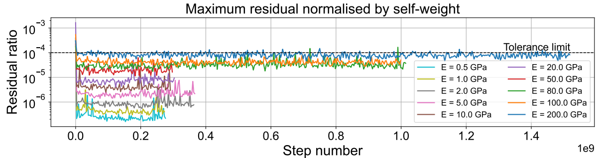
Figure 8: The convergence behaviour during the simulations in Figure 6 where the maximum residual force is normalised by the self-weight of the arch.
