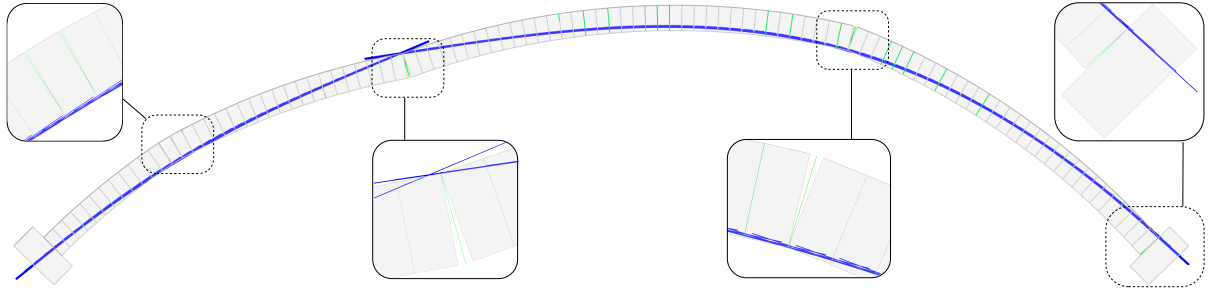
Figure 5: Results of the discrete element analysis using LMGC90. The blue lines indicate the stress resultants.
