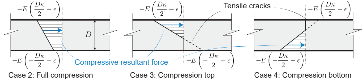
Figure 2: Cases 2, 3 and 4 in (6) and (7) of the cracked elastic arch, only taking into account areas in compression.
