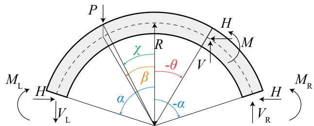
Figure 1: Geometry, loading, reactions, section forces, and notation for the circular arch.
