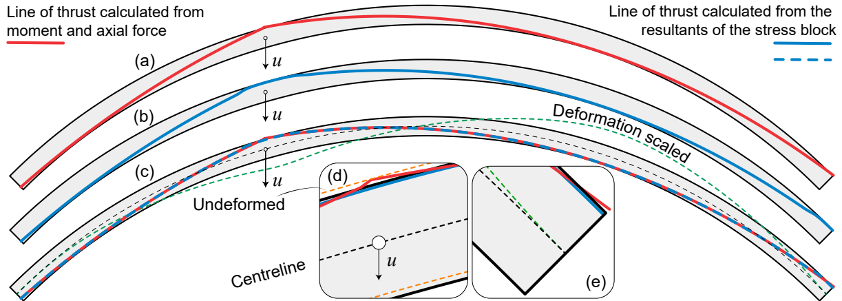
Figure 9: The deformed arch at peak load with E = 20 GPa. In (a), the red curve is the ratio of bending moment to axial force. In (b), the blue line is the resultant of the stress block. In (c), the curves from (a) and (b) are superimposed, and the green dashed curve shows the deformed shape amplified by a factor of 20. Figures (d) and (e) provide zoomed-in views of part of (c), showing both curves in the region of the applied load and right support.
