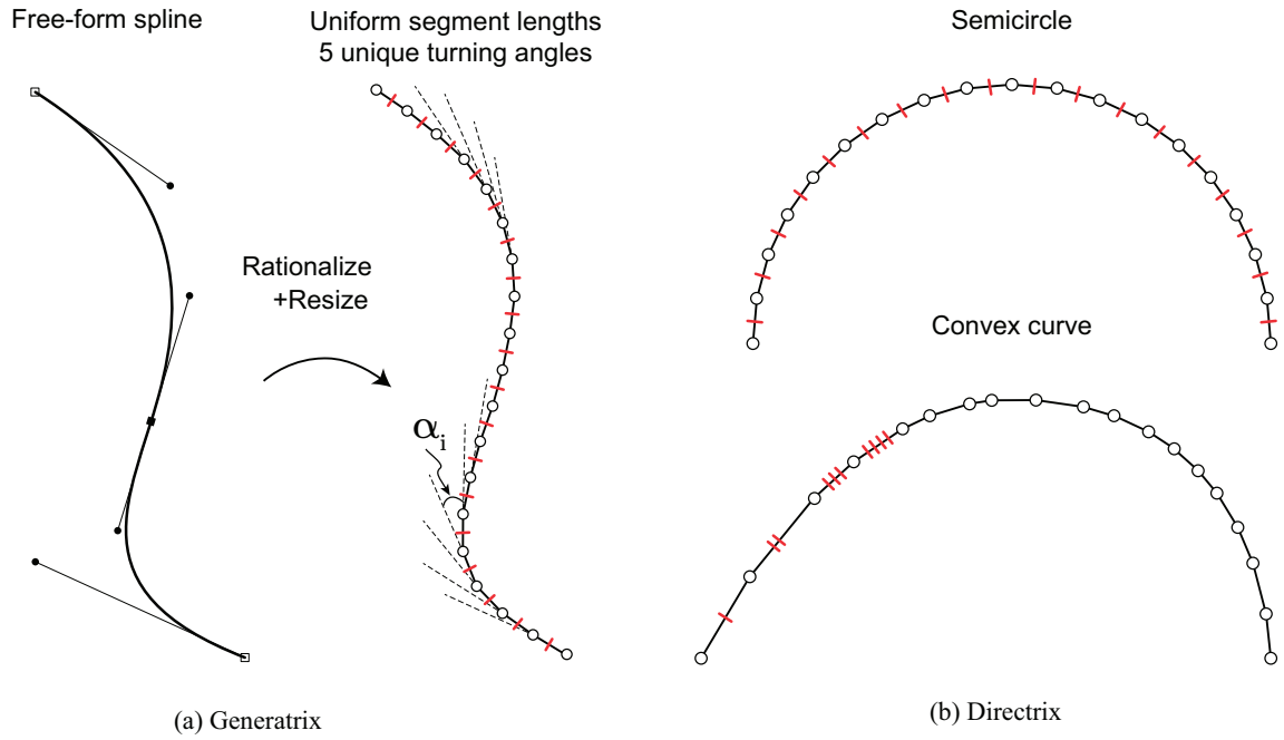
Figure 3: Construction of the guiding curves. (a) Rationalisation of the generatrix from a free-form spline into a polyline with uniform segment lengths and a limited set of turning angles \alpha_i . (b) Isogonal discretisations of two admissible directrices: a semicircle and an arbitrary convex curve.
