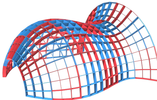
Figure 6: Division of pavilion into 36 assembly zones.
