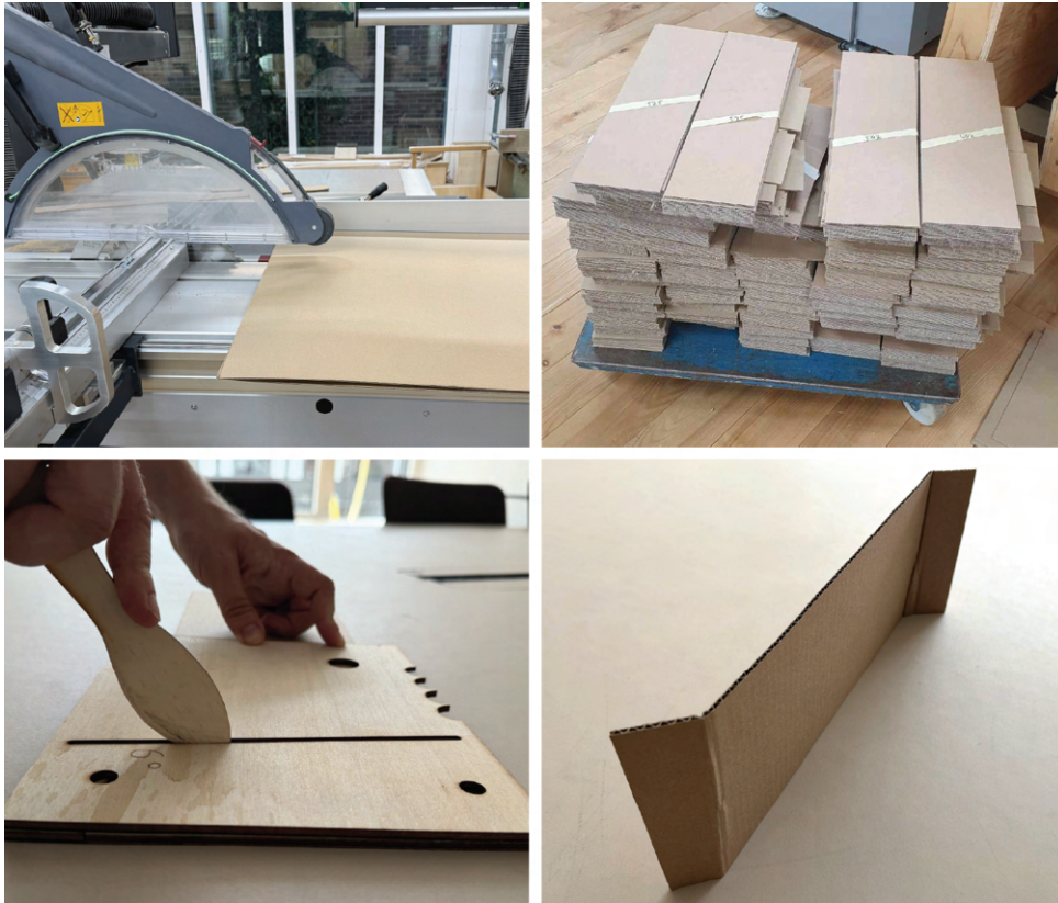
Figure 5: Fabrication sequence from cardboard sheet to finished element. Top left: cutting sheets to size using a circular saw. Top right: batch of elements after cutting. Bottom left: formation of crease lines using a creasing rig. Bottom right: completed element ready for assembly.
