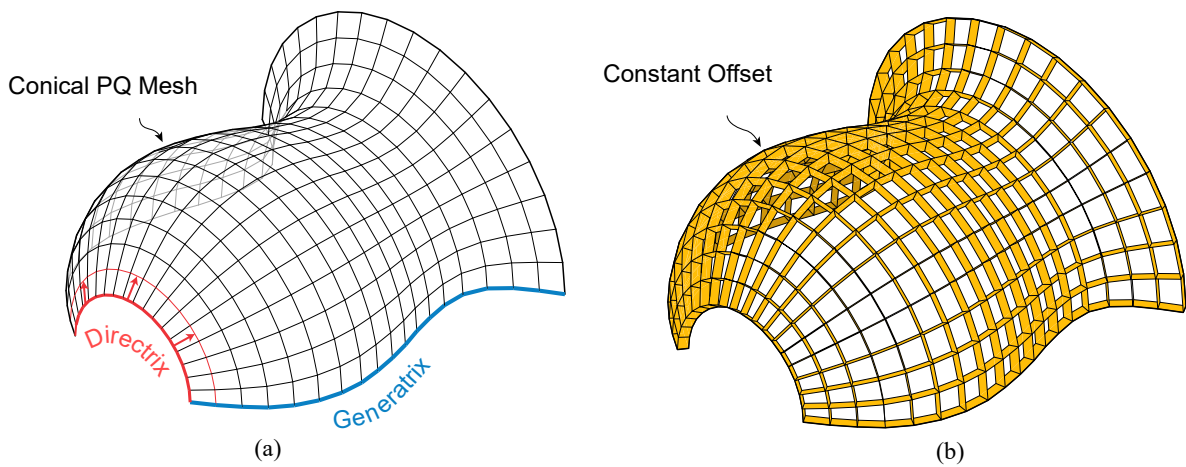
Figure 2: Generation of the grid shell geometry. (a) isogonal moulding surface generated by translating a generatrix along a directrix, (b) the members are found by applying a constant offset.
