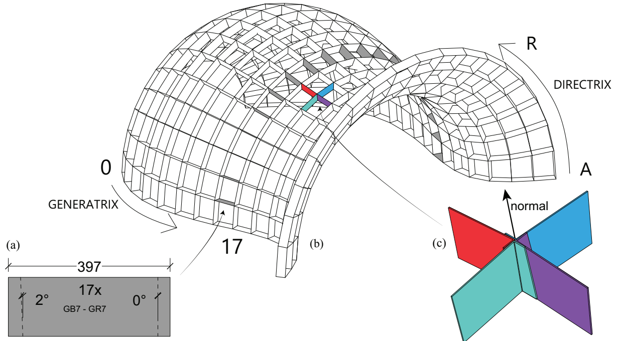
Figure 4: Fabrication information generated from the parametric model. (a) Example member drawing with cutting length, crease angles, label, and quantity. (b) Global member labelling scheme based on generatrix and directrix indices. (c) Node assembly illustrating the integrated folding connection detail between intersecting members.
