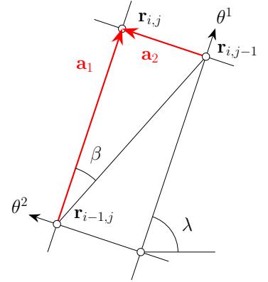
Figure 4: Points in the numerical integration
