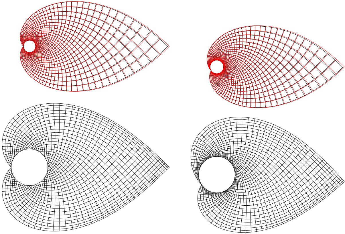
(a) Top: Cantilever as in Michell's paper with load at tip, made of one weightless material, analytic model in red, numerical in black.
