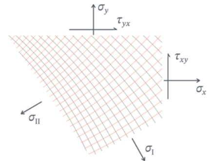
Figure 2: Structural members and Cartesian components of stress and principal stresses in 2 dimensions. One of the principal stresses is positive and the other is negative.
