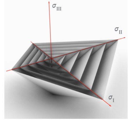
Figure 3: Michell's octahedral contour surfaces of constant \mathcal{M} in principal stress space sliced by the plane \sigma_{III} = 0
