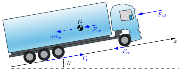
Fig. 1. A free body diagram of a 4 × 8 rigid truck on a road grade, \theta , subject to a rolling resistance force F_{rr} , air drag force F_{ad} , hill climbing force F_{hc} , inertial force m\dot{v}_x , and traction force F_t .
