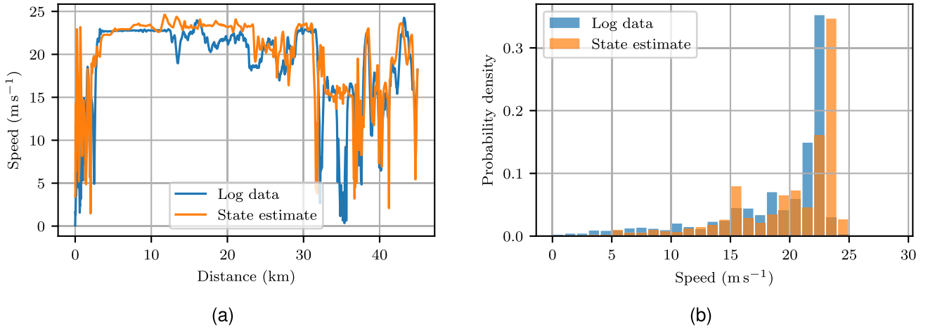
Fig. 2. Figure (a) displays logged vehicle speed (blue) and estimated vehicle speed (orange) over a transport mission. Figure (b) displays the distribution of these speed signals.
