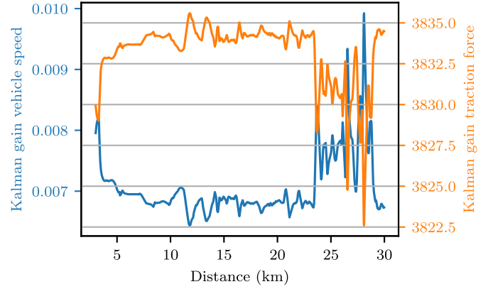
Fig. 3. The figure shows the stationary Kalman gain over a segment of a transport mission.
