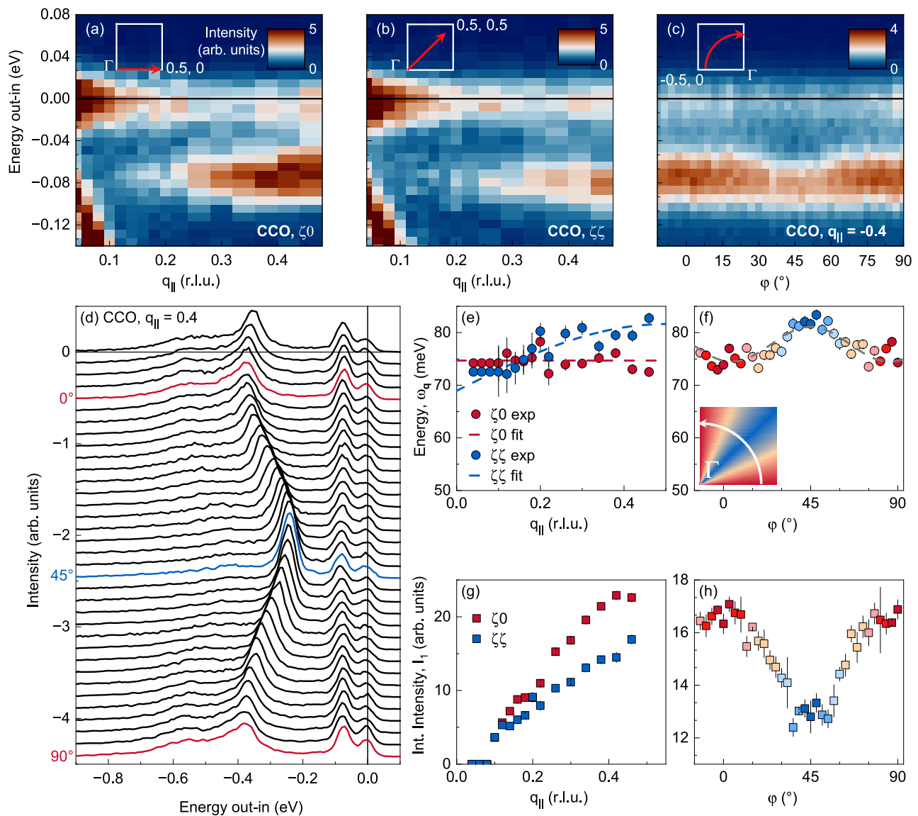
Fig. 5 | RIXS spectra of CaCuO 2 . Experimental RIXS intensity maps along the a ( \zeta, 0 ), b ( \zeta, \zeta ) and c azimuth path. The trajectories in the reciprocal space are indicated in the insets. d A stack of RIXS spectra in the \phi scan. The red and blue curves indicate spectra at (-0.4, 0) , (0, 0.4) and (-0.4/\sqrt{2}, 0.4/\sqrt{2}) in r.l.u., respectively. e, f Experimental breathing phonon energy (symbols) with q_{||} along the same path as in a , b and c . The inset colormap in f indicates the adopted color- q_{||}
