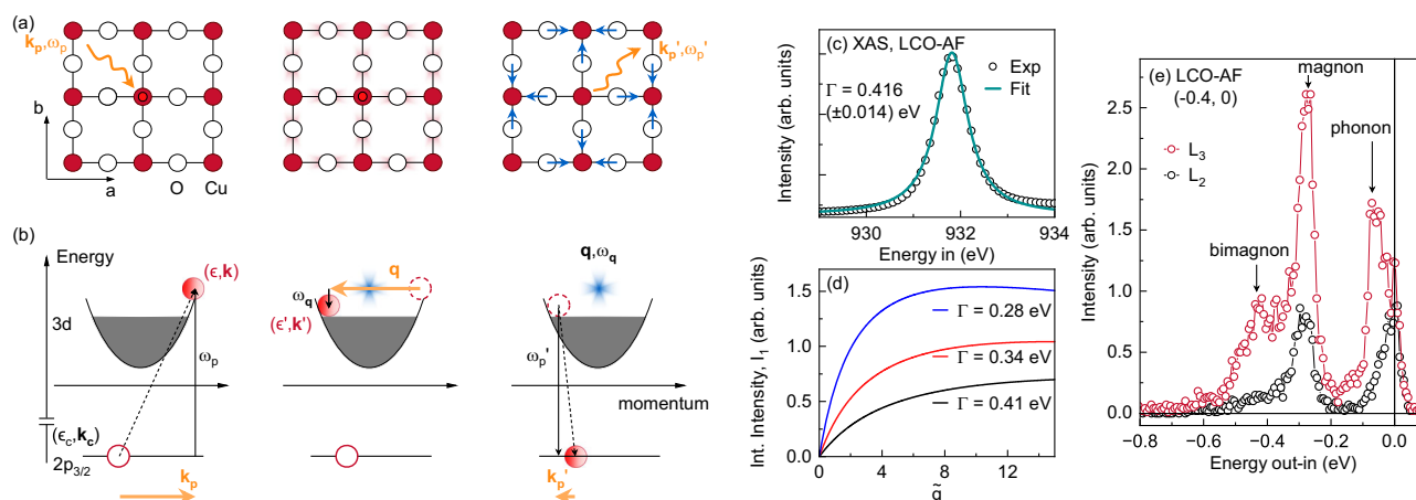
Fig. 1 | Features of phonon excitation in RIXS. A scheme of phonon generation in RIXS process at the Cu L_3 edge in (a) real and (b) reciprocal spaces. Here, \mathbf{k}_p, \omega_p ( \mathbf{k}', \omega' ) are the wavevector and energy of the incoming (outgoing) photon; \mathbf{k}_c, \epsilon_c are the wavevector and energy of the core-hole; \mathbf{k}, \epsilon ( \mathbf{k}', \epsilon' ) are the wavevector and energy of the photo-excited electron before (after) the phonon generation; \mathbf{q}, \omega_q are the wavevector and energy of the created phonon. For the conservation of the momentum and energy: \mathbf{k}' = \mathbf{k} + \mathbf{q} , \mathbf{k}' = \mathbf{k}_p + \mathbf{q} , \omega_q = \omega_p - \omega' = \epsilon - \epsilon' ,
