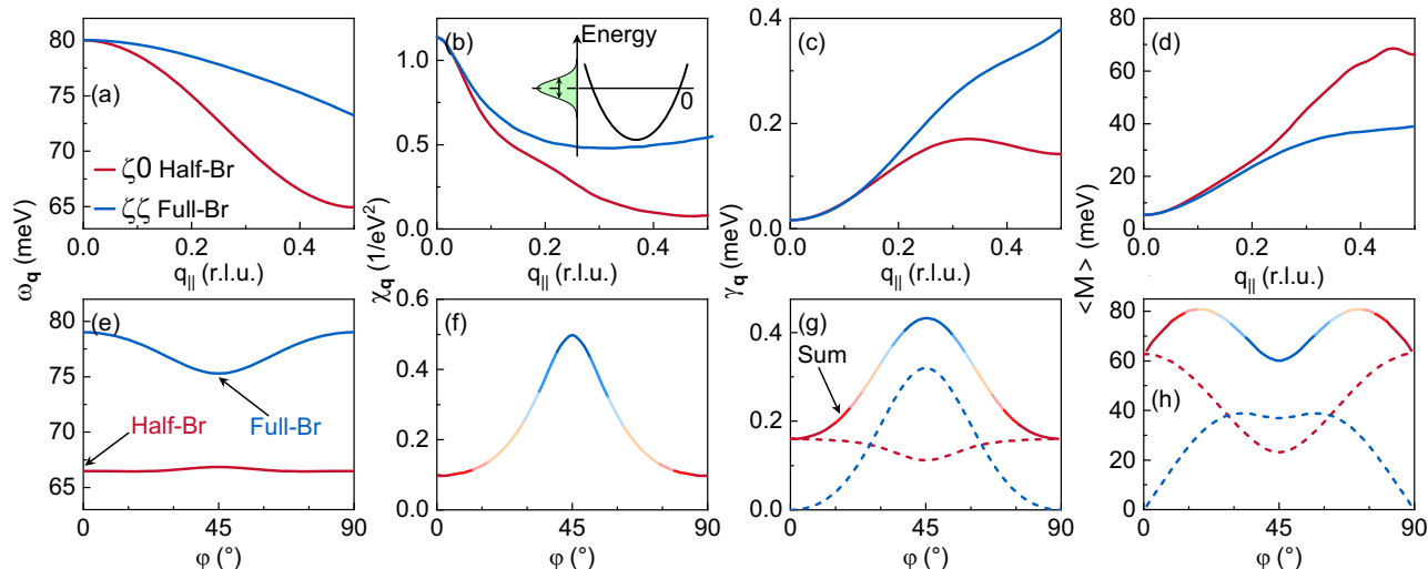
Fig. 10 | EPC with DFT. a–d The EPC quantities calculated with DFT along a–d the (\zeta,0) , (\zeta,\zeta) and (e–h) \varphi ( q_{\parallel} = 0.4 ) lines. The q_{\parallel} -dependence of the energy of the bond-stretching mode is in agreement with previous INS measurements 99–102 . The inset in (b) shows a Gaussian region around the Fermi level considered in our DFT calculations. For the (\zeta,0) and (\zeta,\zeta) scans, the red and blue lines correspond to the
